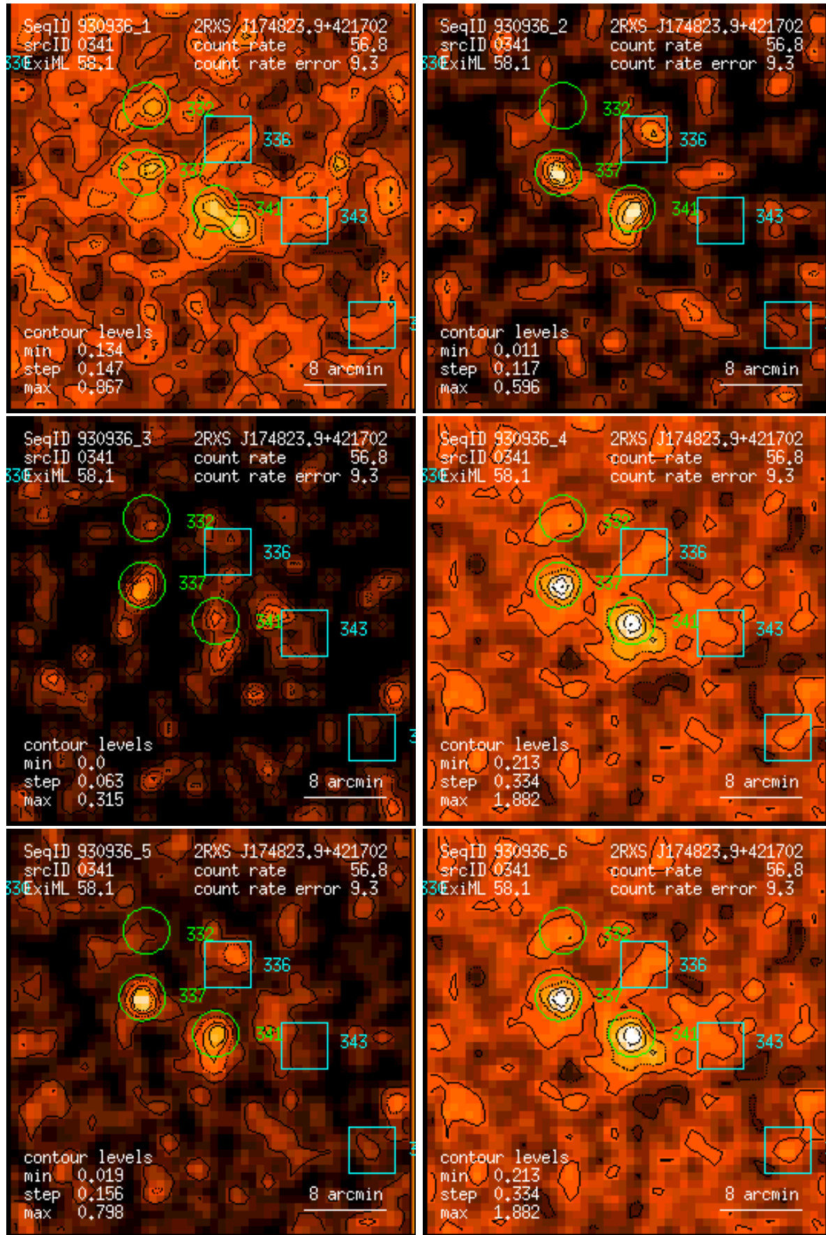
Figure 341: RASS 930936: detection 0341: band rate images, Gaussian filter: (1) PSPC channels 11 – 41, (2) 52 – 90, (3) 91 – 201, (4) 11 – 235, (5) 52 – 201, (6) 11 – 201. Broad band rates in counts/ks. Band rate contour levels in counts/ks/arcmin 2 .
