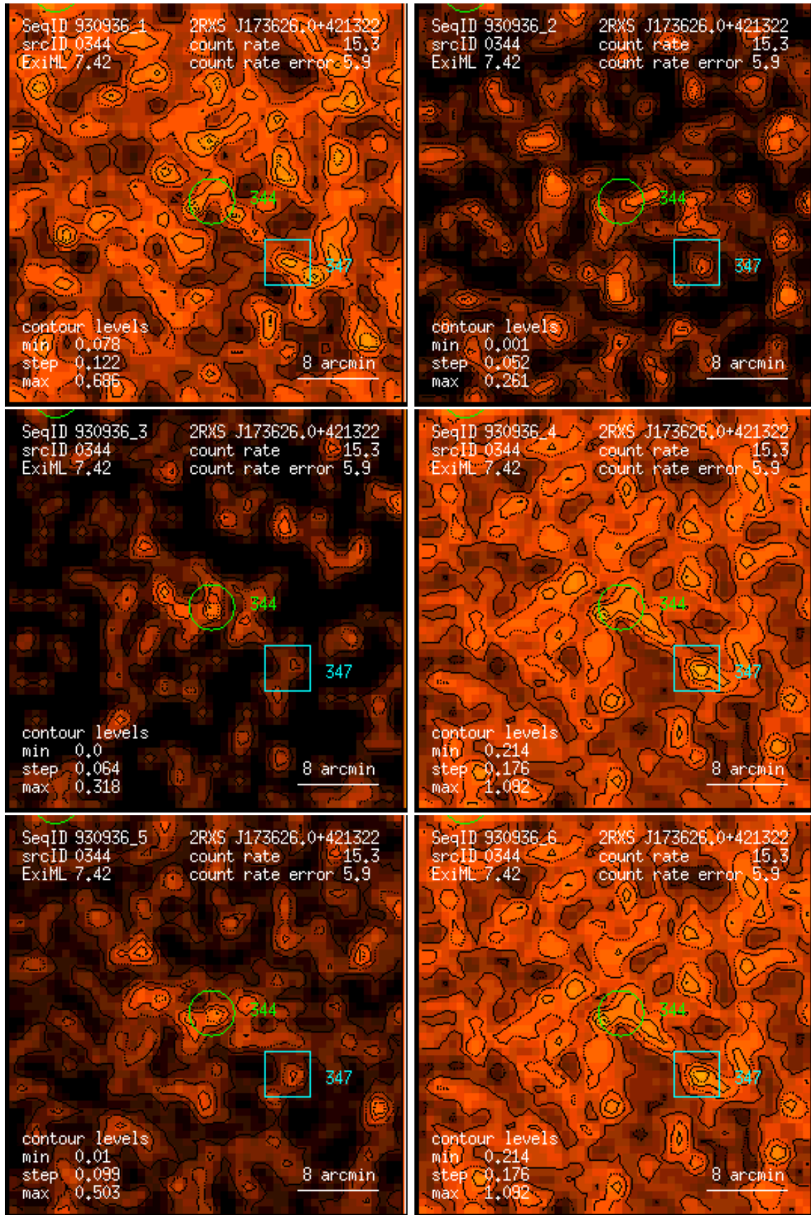
Figure 344: RASS 930936: detection 0344: band rate images, Gaussian filter: (1) PSPC channels 11 – 41, (2) 52 – 90, (3) 91 – 201, (4) 11 – 235, (5) 52 – 201, (6) 11 – 201. Broad band rates in counts/ks. Band rate contour levels in counts/ks/arcmin 2 .
