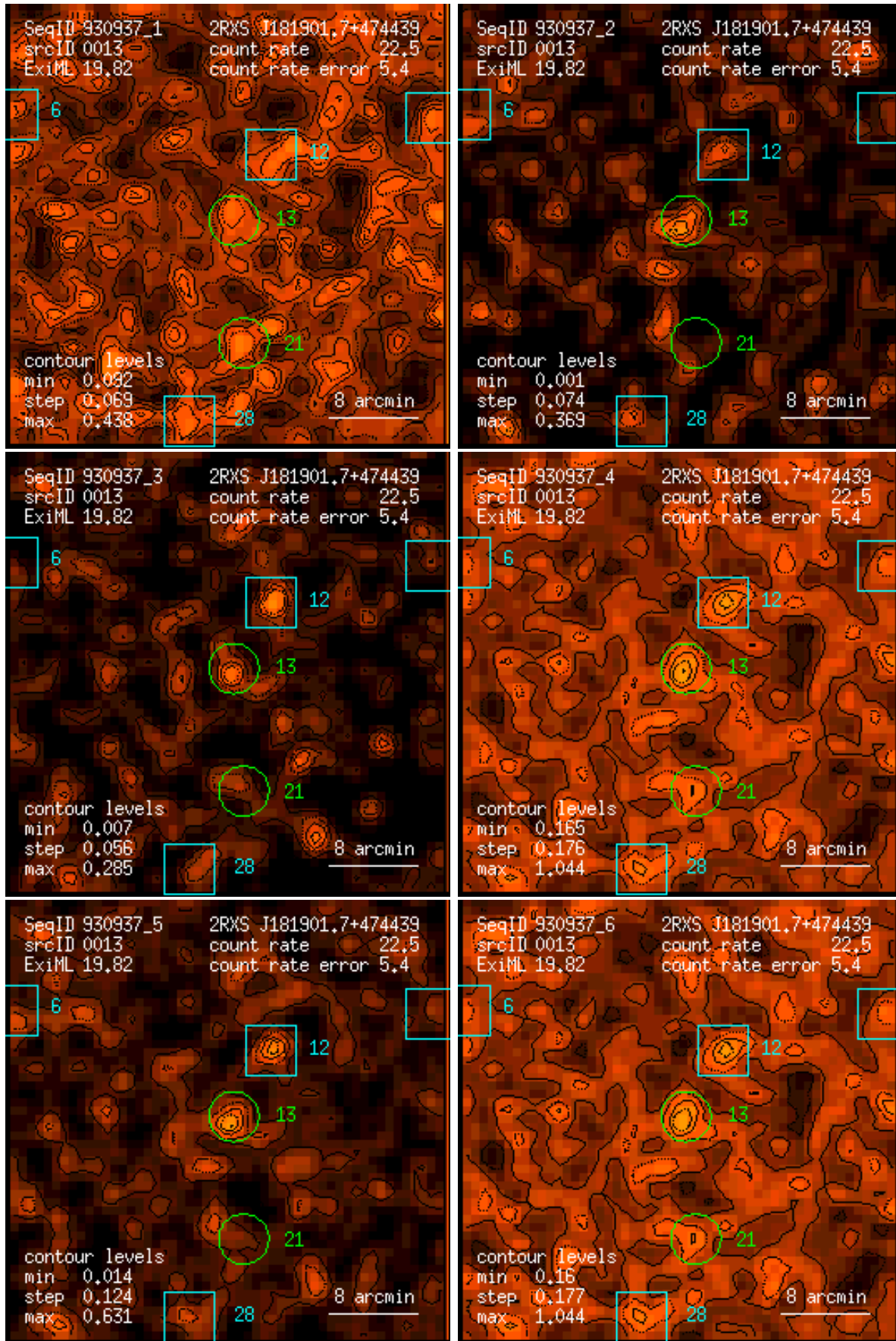
Figure 13: RASS 930937: detection 0013: band rate images, Gaussian filter: (1) PSPC channels 11 – 41, (2) 52 – 90, (3) 91 – 201, (4) 11 – 235, (5) 52 – 201, (6) 11 – 201. Broad band rates in counts/ks. Band rate contour levels in counts/ks/arcmin 2 .
