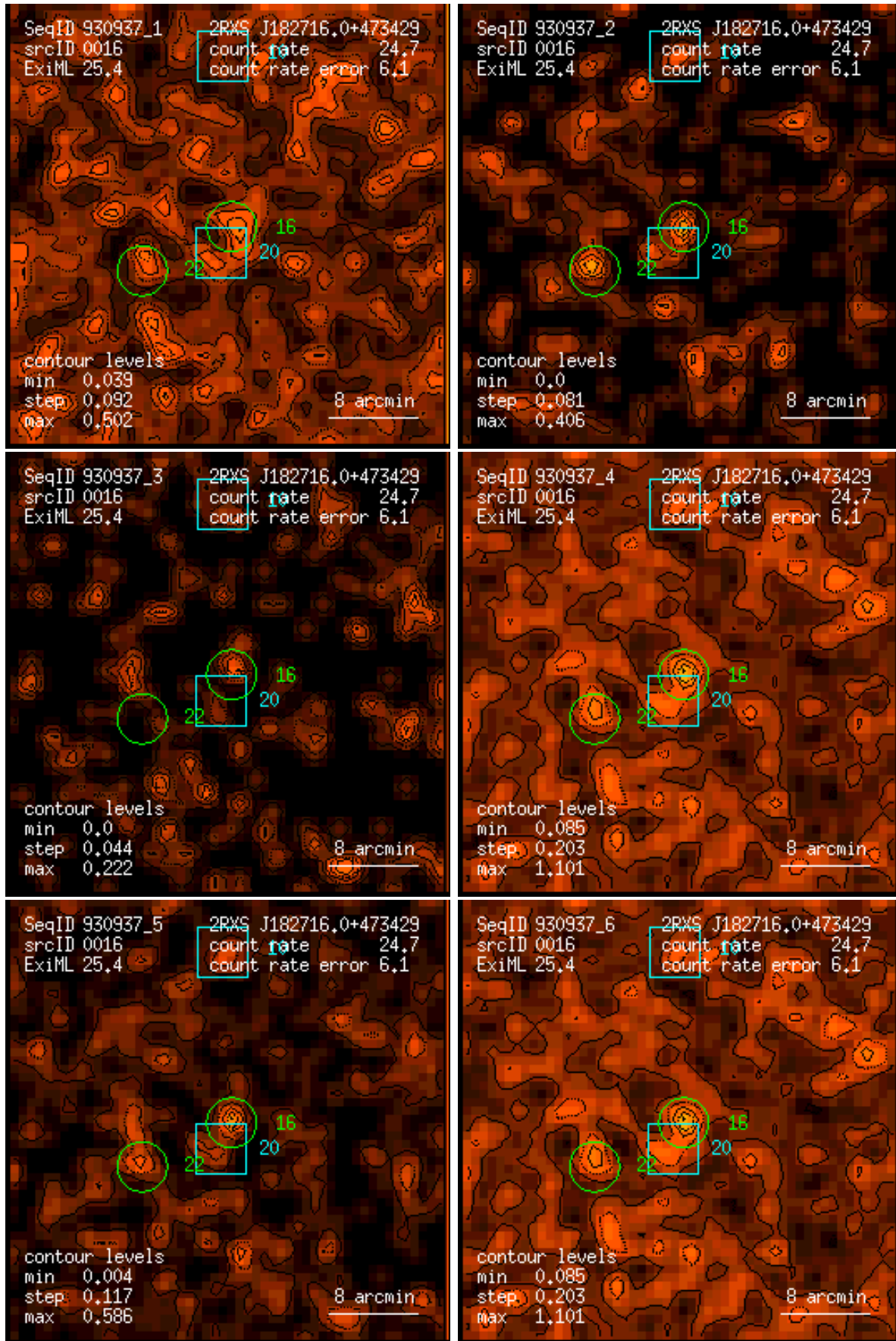
Figure 16: RASS 930937: detection 0016: band rate images, Gaussian filter: (1) PSPC channels 11 – 41, (2) 52 – 90, (3) 91 – 201, (4) 11 – 235, (5) 52 – 201, (6) 11 – 201. Broad band rates in counts/ks. Band rate contour levels in counts/ks/arcmin 2 .
