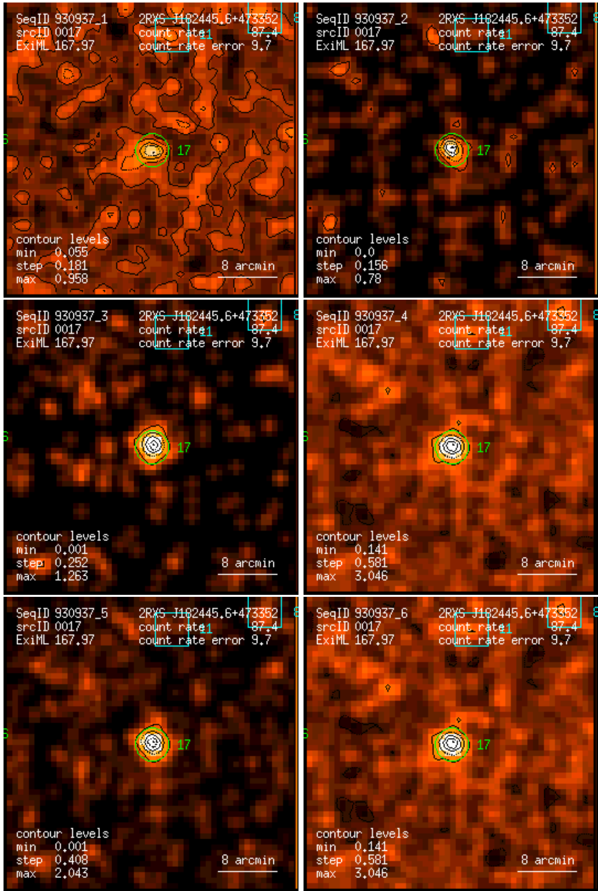
Figure 17: RASS 930937: detection 0017: band rate images, Gaussian filter: (1) PSPC channels 11 – 41, (2) 52 – 90, (3) 91 – 201, (4) 11 – 235, (5) 52 – 201, (6) 11 – 201. Broad band rates in counts/ks. Band rate contour levels in counts/ks/arcmin 2 .
