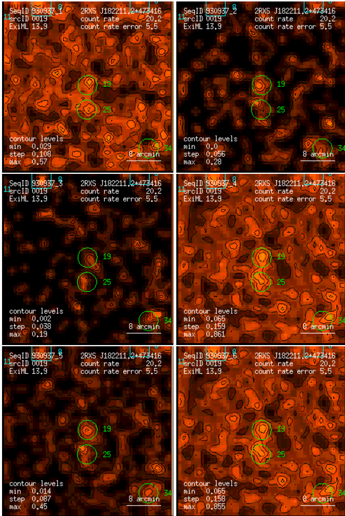
Figure 19: RASS 930937: detection 0019: band rate images, Gaussian filter: (1) PSPC channels 11 – 41, (2) 52 – 90, (3) 91 – 201, (4) 11 – 235, (5) 52 – 201, (6) 11 – 201. Broad band rates in counts/ks. Band rate contour levels in counts/ks/arcmin 2 .
