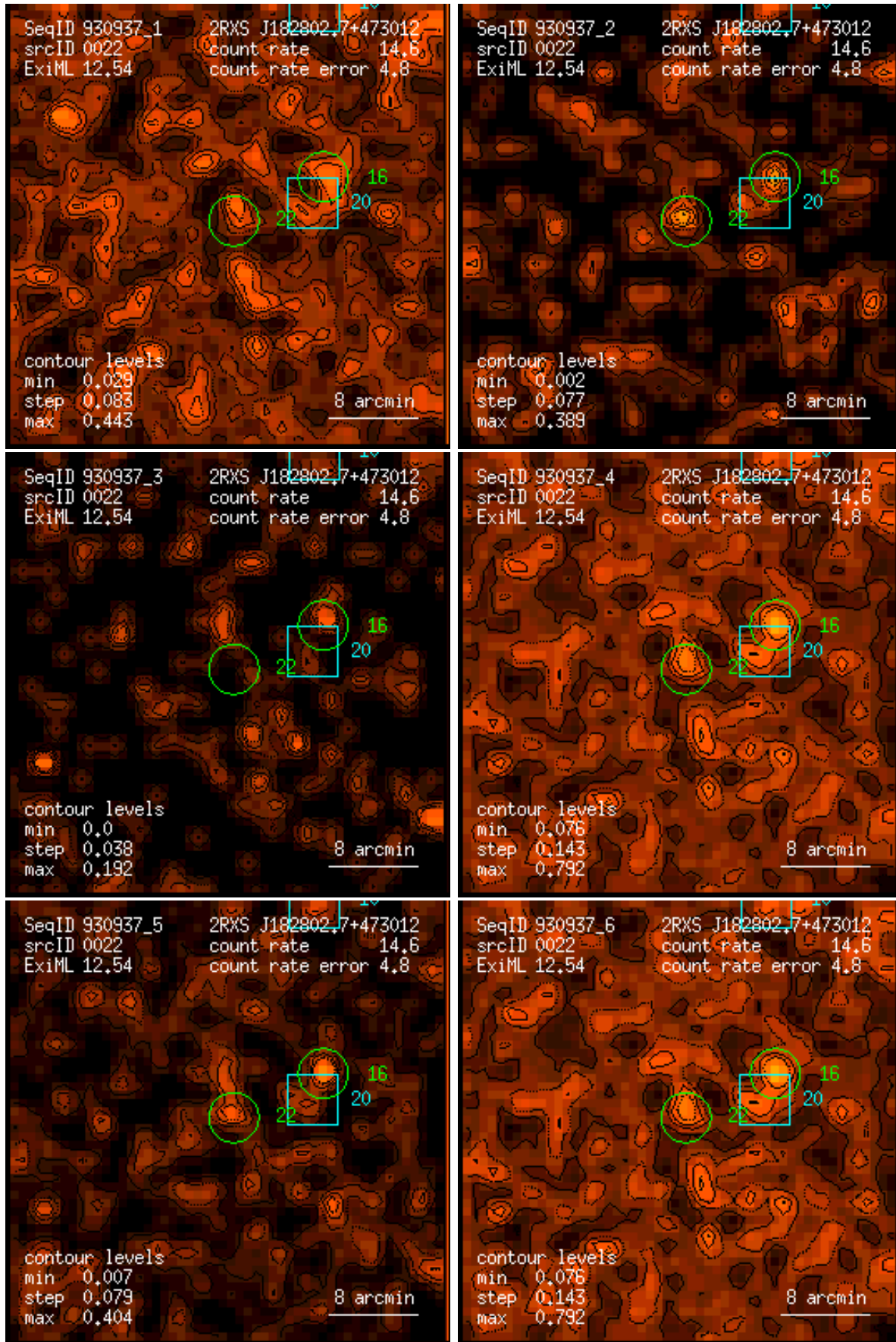
Figure 22: RASS 930937: detection 0022: band rate images, Gaussian filter: (1) PSPC channels 11 – 41, (2) 52 – 90, (3) 91 – 201, (4) 11 – 235, (5) 52 – 201, (6) 11 – 201. Broad band rates in counts/ks. Band rate contour levels in counts/ks/arcmin 2 .
