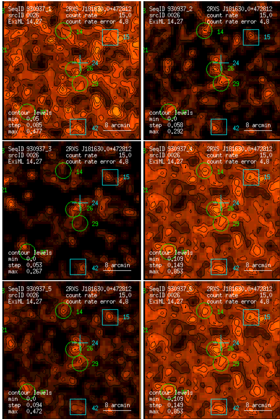
Figure 26: RASS 930937: detection 0026: band rate images, Gaussian filter: (1) PSPC channels 11 – 41, (2) 52 – 90, (3) 91 – 201, (4) 11 – 235, (5) 52 – 201, (6) 11 – 201. Broad band rates in counts/ks. Band rate contour levels in counts/ks/arcmin 2 .
