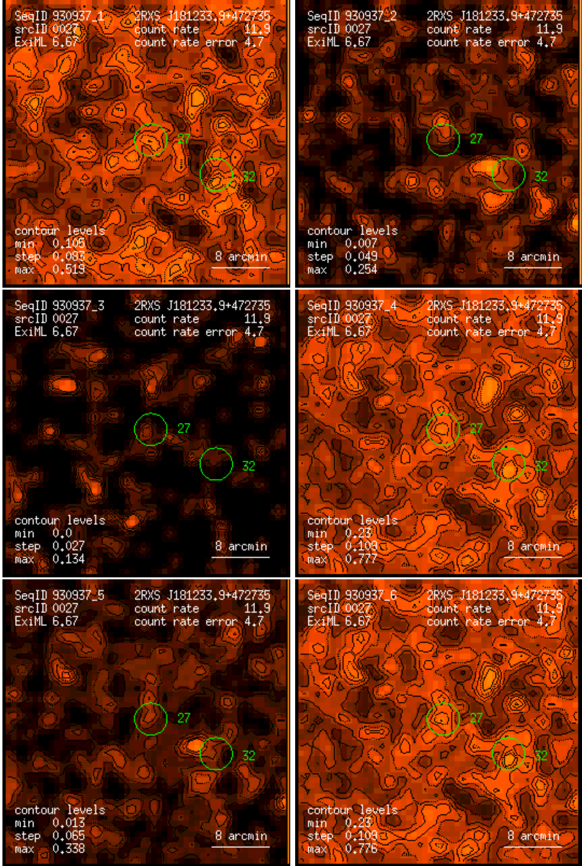
Figure 27: RASS 930937: detection 0027: band rate images, Gaussian filter: (1) PSPC channels 11 – 41, (2) 52 – 90, (3) 91 – 201, (4) 11 – 235, (5) 52 – 201, (6) 11 – 201. Broad band rates in counts/ks. Band rate contour levels in counts/ks/arcmin 2 .
