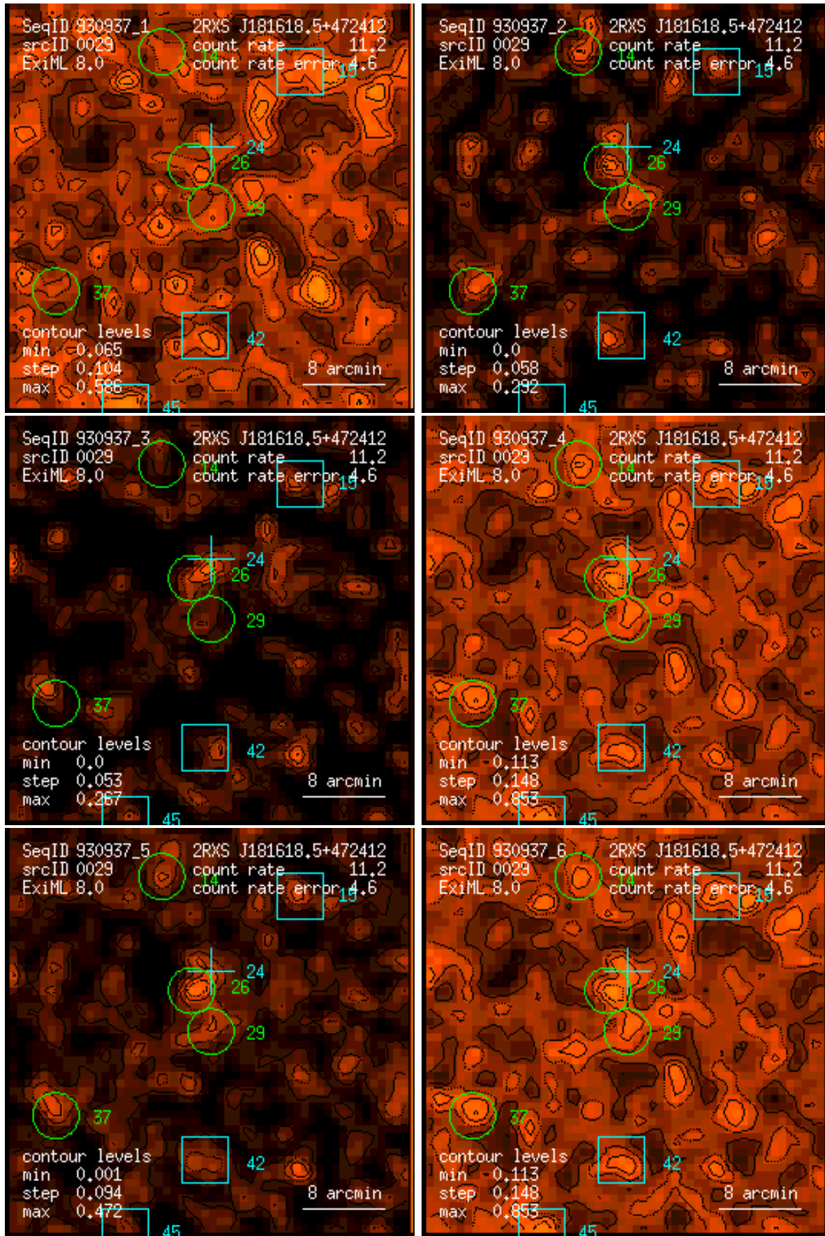
Figure 29: RASS 930937: detection 0029: band rate images, Gaussian filter: (1) PSPC channels 11 – 41, (2) 52 – 90, (3) 91 – 201, (4) 11 – 235, (5) 52 – 201, (6) 11 – 201. Broad band rates in counts/ks. Band rate contour levels in counts/ks/arcmin 2 .
