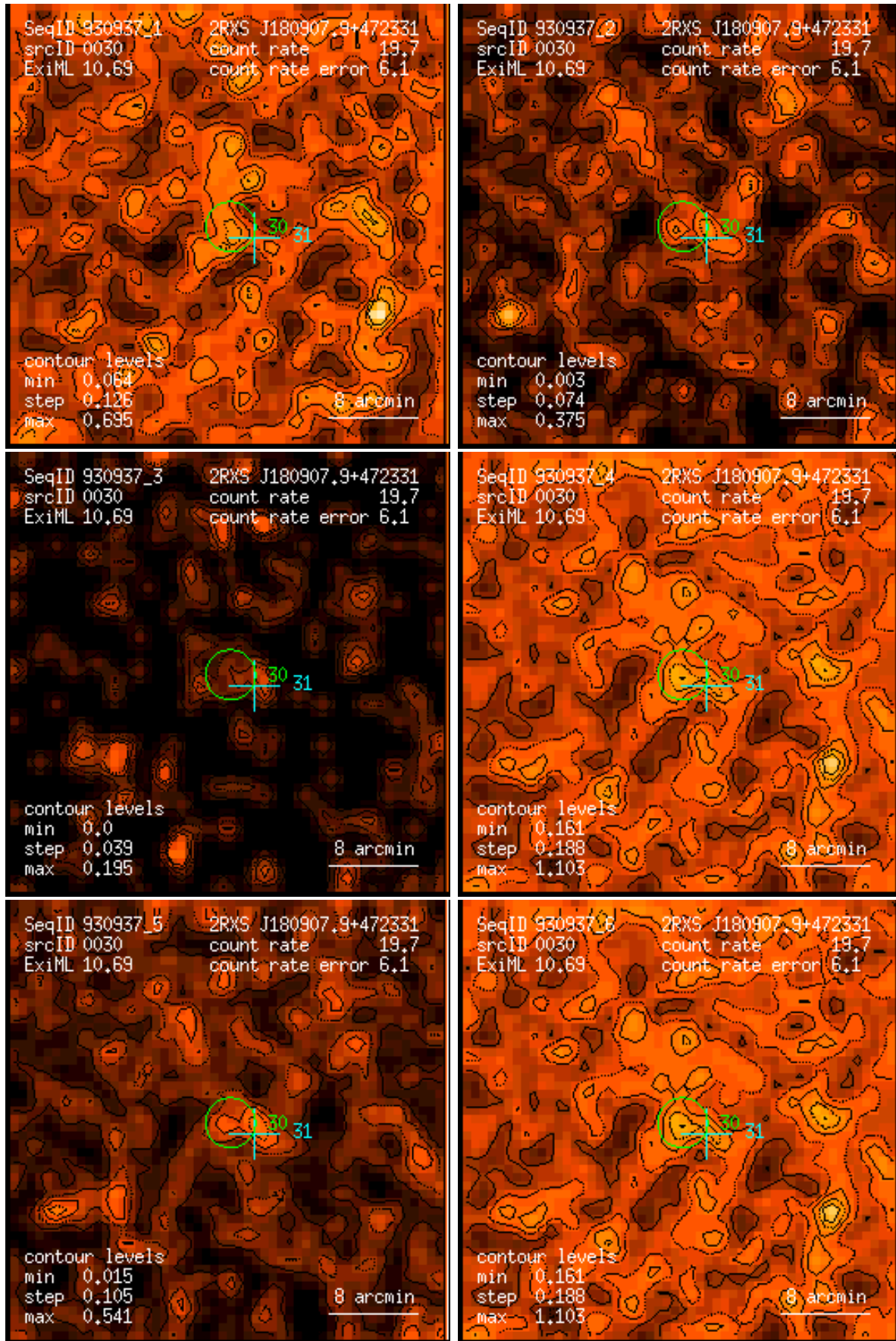
Figure 30: RASS 930937: detection 0030: band rate images, Gaussian filter: (1) PSPC channels 11 – 41, (2) 52 – 90, (3) 91 – 201, (4) 11 – 235, (5) 52 – 201, (6) 11 – 201. Broad band rates in counts/ks. Band rate contour levels in counts/ks/arcmin 2 .
