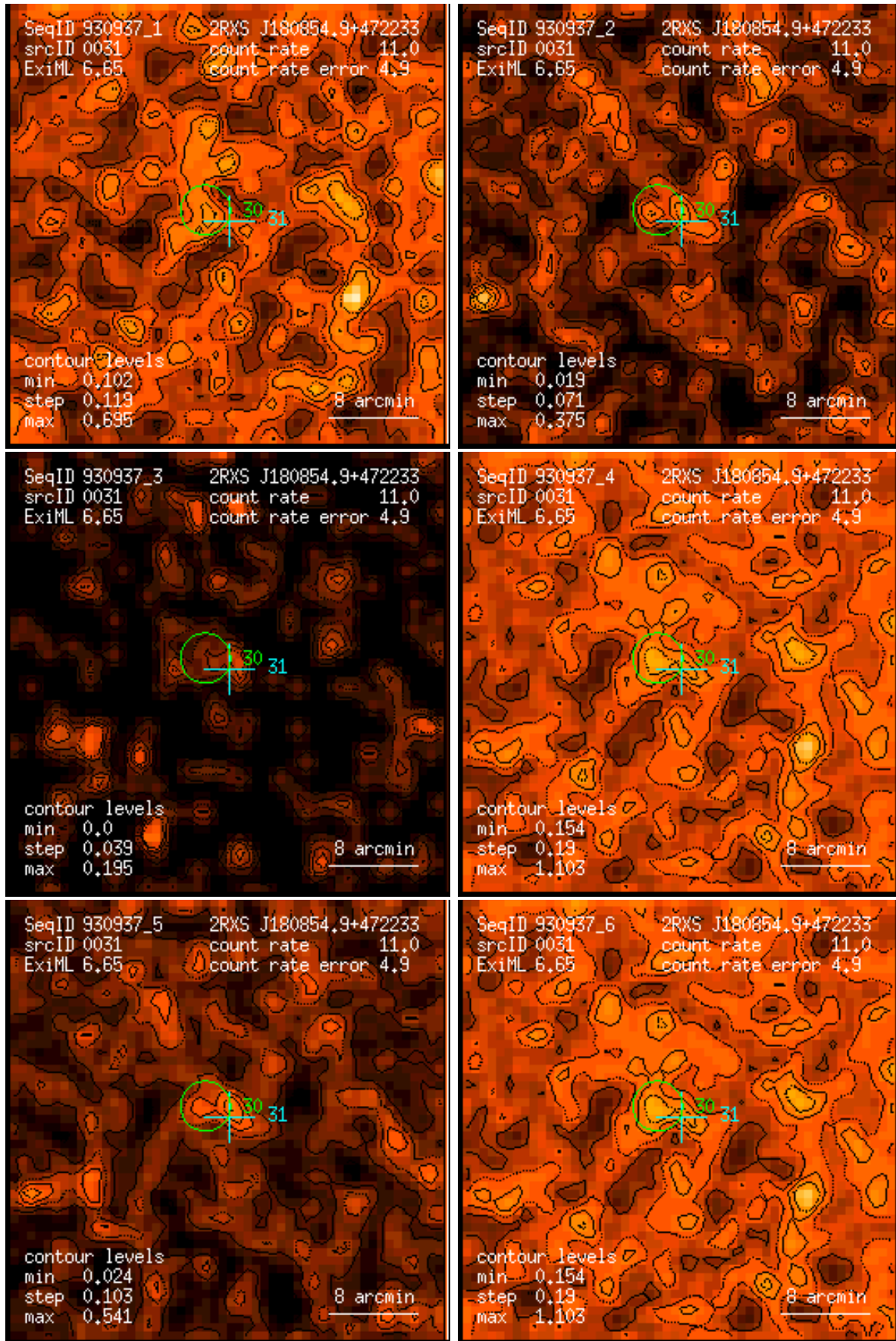
Figure 31: RASS 930937: detection 0031: band rate images, Gaussian filter: (1) PSPC channels 11 – 41, (2) 52 – 90, (3) 91 – 201, (4) 11 – 235, (5) 52 – 201, (6) 11 – 201. Broad band rates in counts/ks. Band rate contour levels in counts/ks/arcmin 2 .
