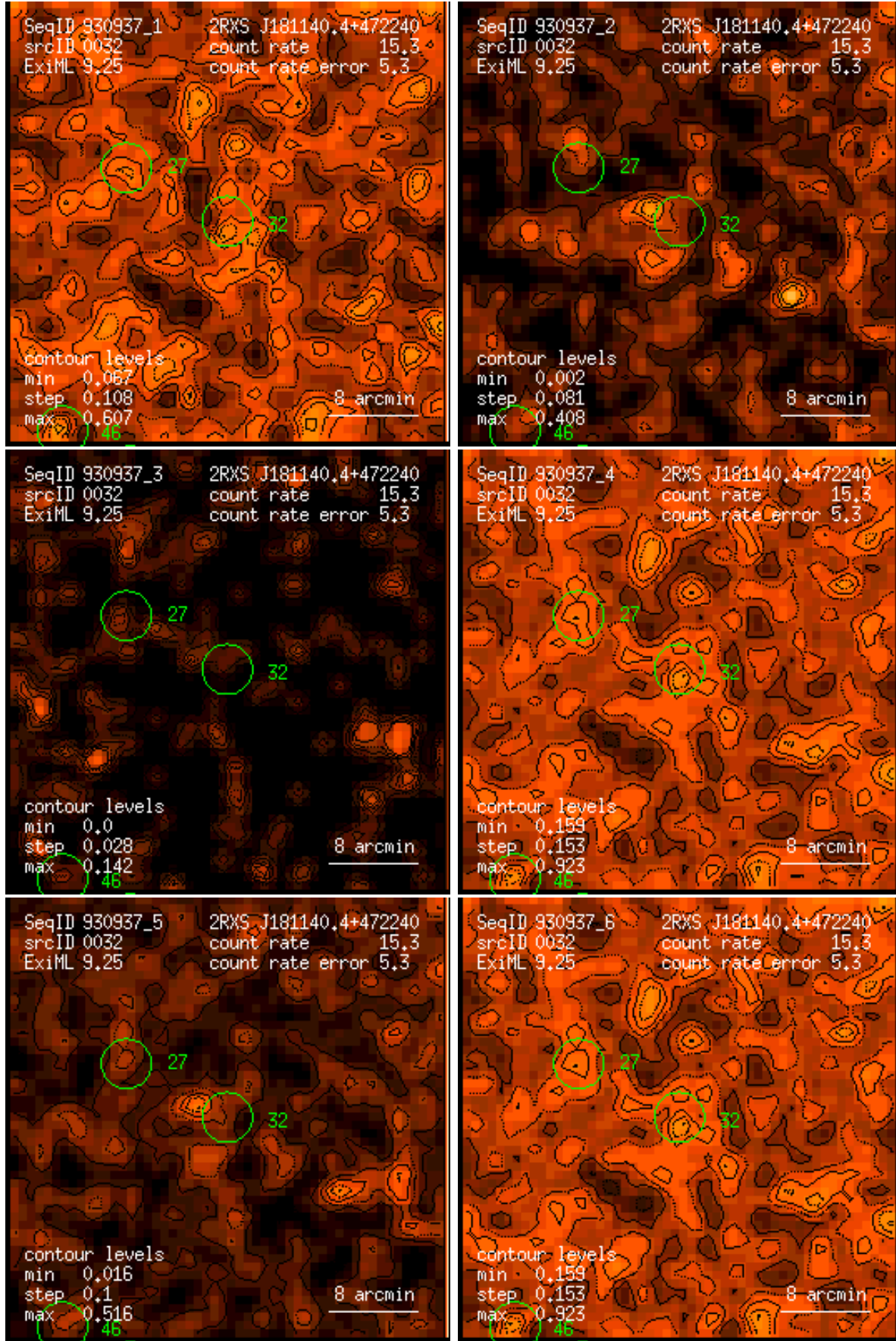
Figure 32: RASS 930937: detection 0032: band rate images, Gaussian filter: (1) PSPC channels 11 – 41, (2) 52 – 90, (3) 91 – 201, (4) 11 – 235, (5) 52 – 201, (6) 11 – 201. Broad band rates in counts/ks. Band rate contour levels in counts/ks/arcmin 2 .
