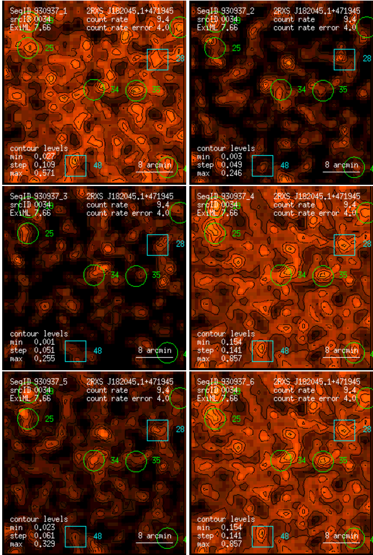
Figure 34: RASS 930937: detection 0034: band rate images, Gaussian filter: (1) PSPC channels 11 – 41, (2) 52 – 90, (3) 91 – 201, (4) 11 – 235, (5) 52 – 201, (6) 11 – 201. Broad band rates in counts/ks. Band rate contour levels in counts/ks/arcmin 2 .
