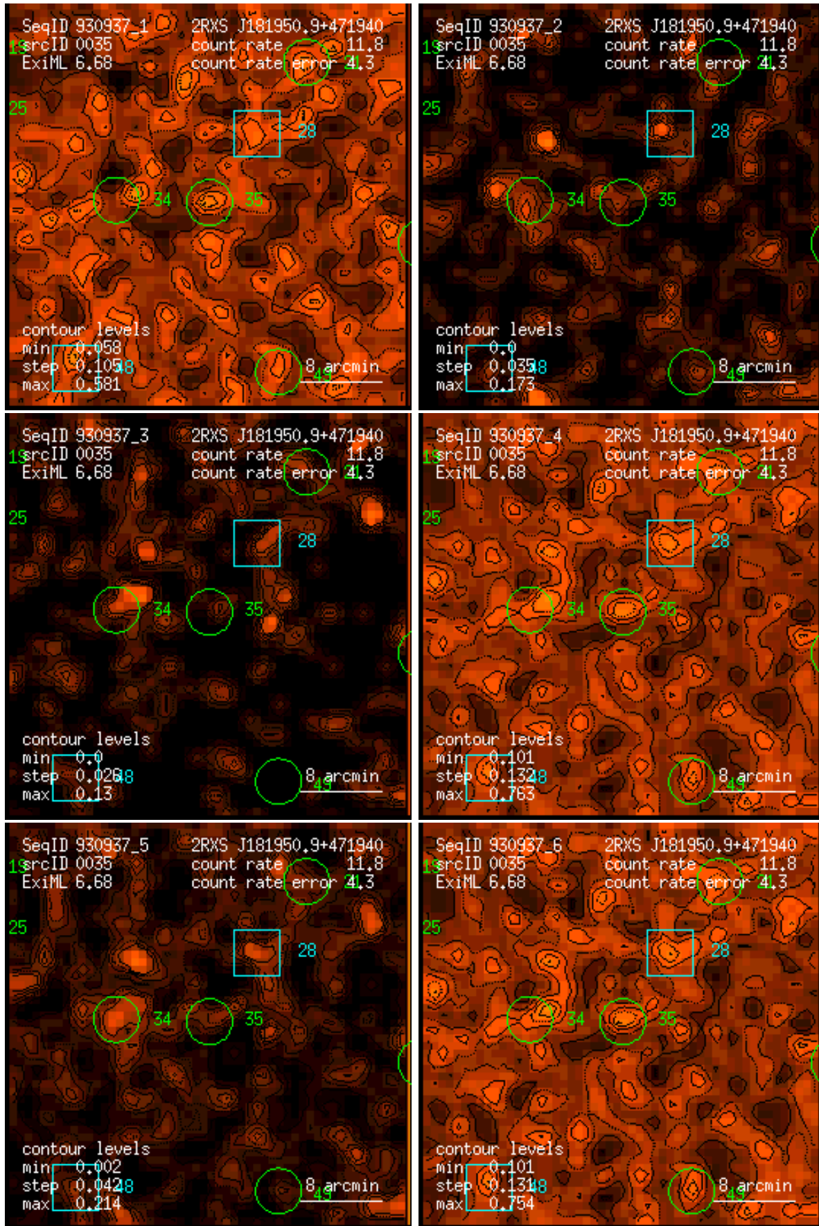
Figure 35: RASS 930937: detection 0035: band rate images, Gaussian filter: (1) PSPC channels 11 – 41, (2) 52 – 90, (3) 91 – 201, (4) 11 – 235, (5) 52 – 201, (6) 11 – 201. Broad band rates in counts/ks. Band rate contour levels in counts/ks/arcmin 2 .
