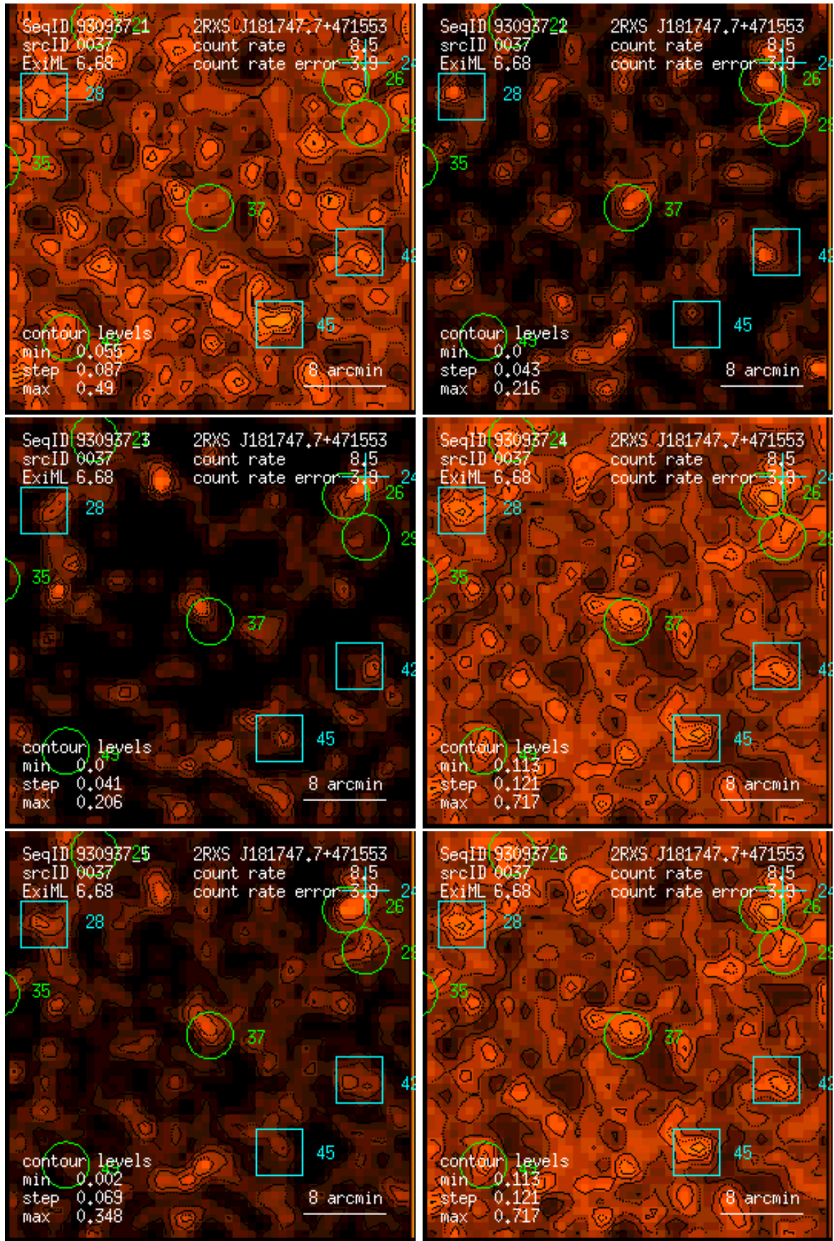
Figure 37: RASS 930937: detection 0037: band rate images, Gaussian filter: (1) PSPC channels 11 – 41, (2) 52 – 90, (3) 91 – 201, (4) 11 – 235, (5) 52 – 201, (6) 11 – 201. Broad band rates in counts/ks. Band rate contour levels in counts/ks/arcmin 2 .
