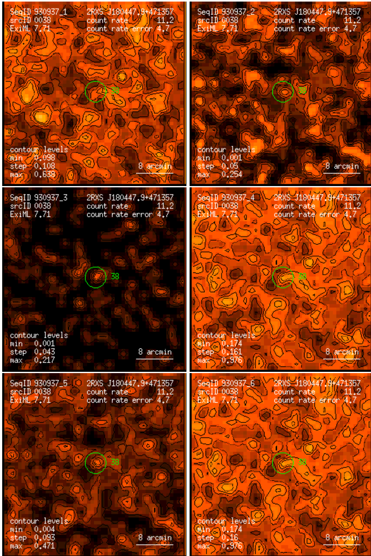
Figure 38: RASS 930937: detection 0038: band rate images, Gaussian filter: (1) PSPC channels 11 – 41, (2) 52 – 90, (3) 91 – 201, (4) 11 – 235, (5) 52 – 201, (6) 11 – 201. Broad band rates in counts/ks. Band rate contour levels in counts/ks/arcmin 2 .
