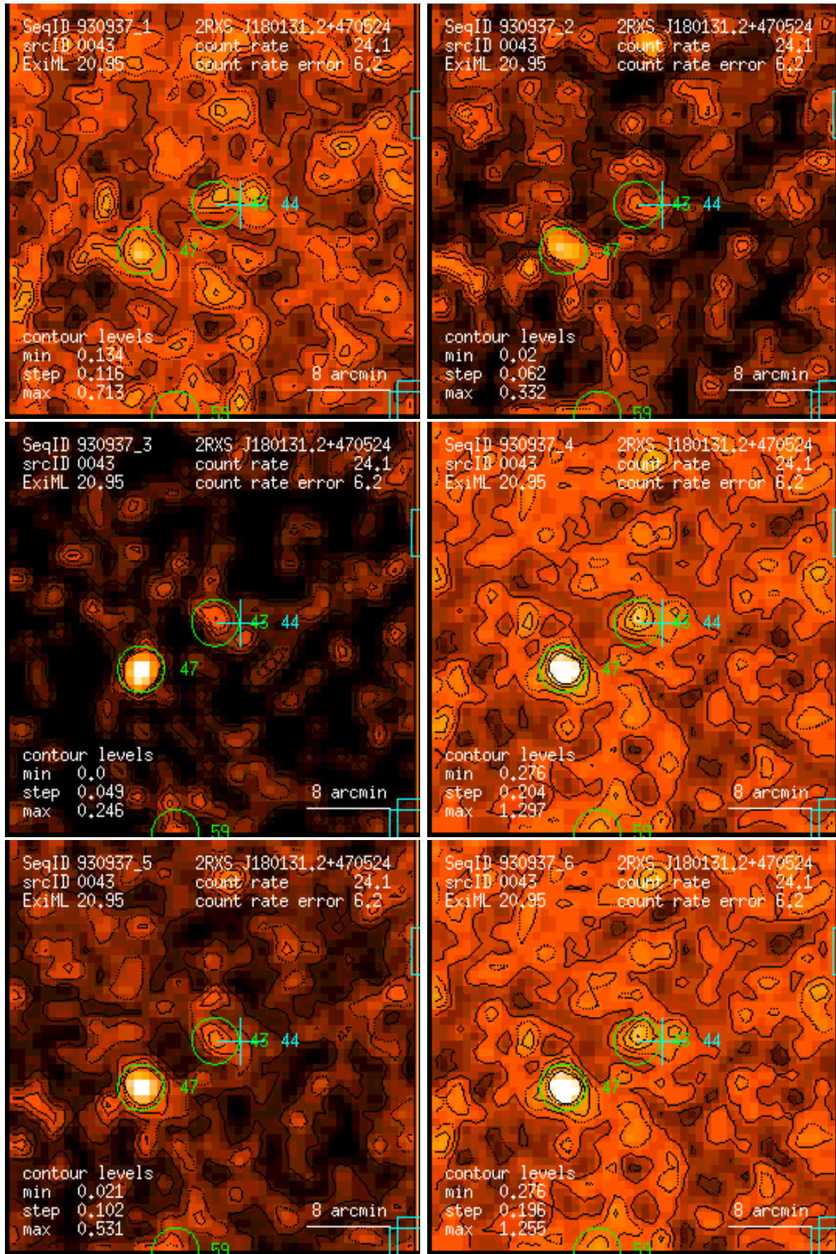
Figure 43: RASS 930937: detection 0043: band rate images, Gaussian filter: (1) PSPC channels 11 – 41, (2) 52 – 90, (3) 91 – 201, (4) 11 – 235, (5) 52 – 201, (6) 11 – 201. Broad band rates in counts/ks. Band rate contour levels in counts/ks/arcmin 2 .
