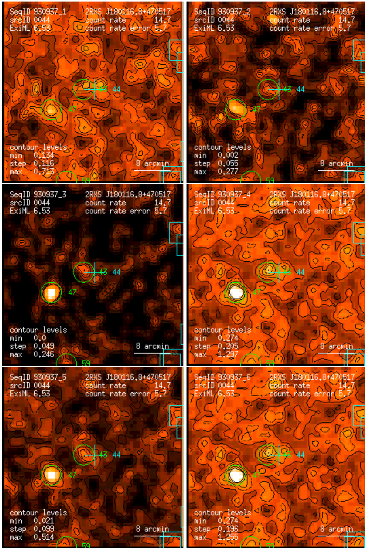
Figure 44: RASS 930937: detection 0044: band rate images, Gaussian filter: (1) PSPC channels 11 – 41, (2) 52 – 90, (3) 91 – 201, (4) 11 – 235, (5) 52 – 201, (6) 11 – 201. Broad band rates in counts/ks. Band rate contour levels in counts/ks/arcmin 2 .
