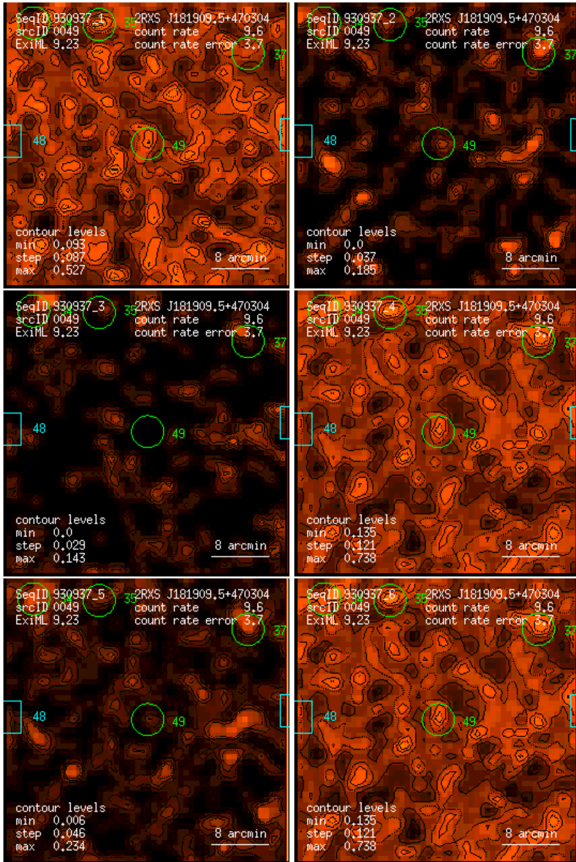
Figure 49: RASS 930937: detection 0049: band rate images, Gaussian filter: (1) PSPC channels 11 – 41, (2) 52 – 90, (3) 91 – 201, (4) 11 – 235, (5) 52 – 201, (6) 11 – 201. Broad band rates in counts/ks. Band rate contour levels in counts/ks/arcmin 2 .
