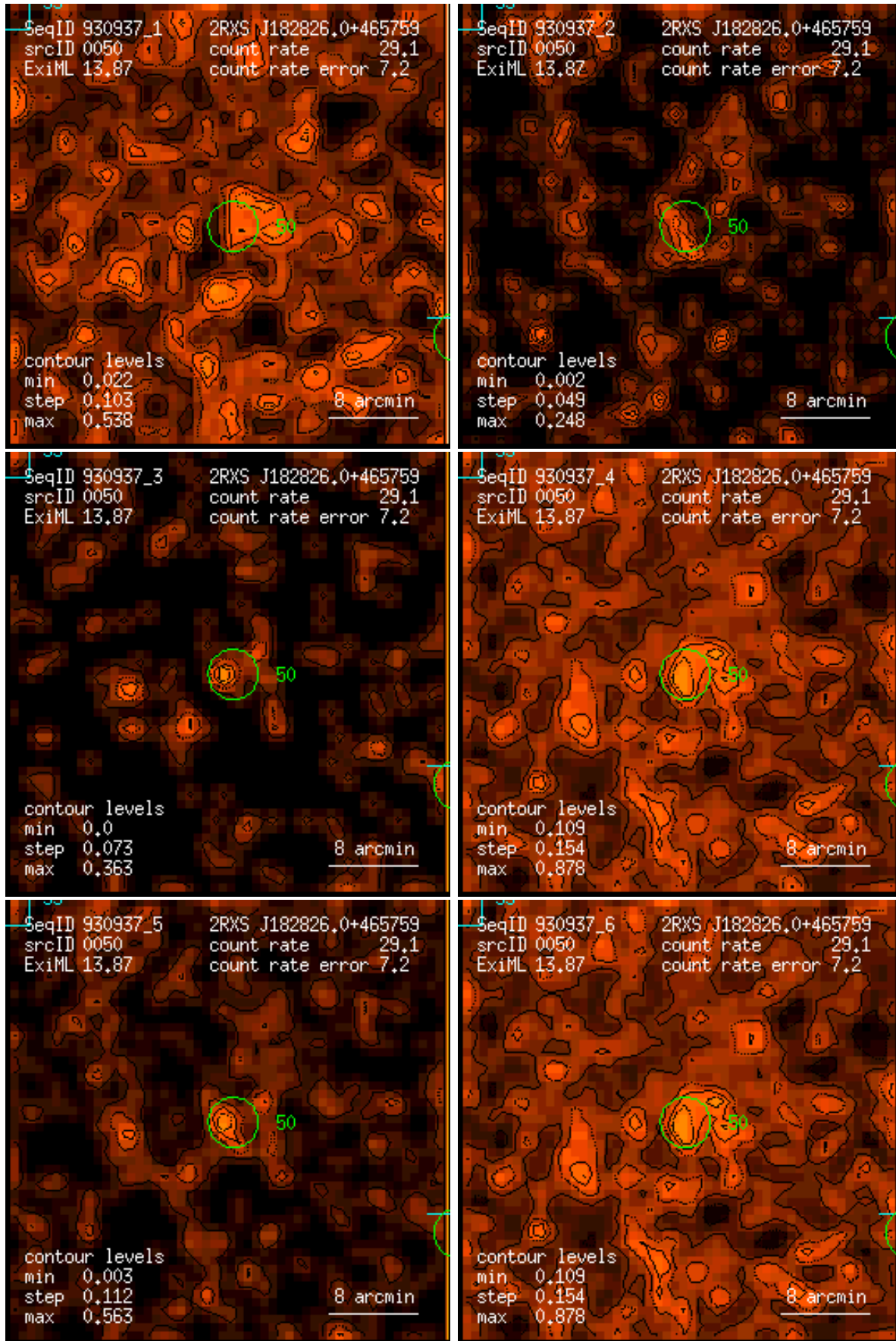
Figure 50: RASS 930937: detection 0050: band rate images, Gaussian filter: (1) PSPC channels 11 – 41, (2) 52 – 90, (3) 91 – 201, (4) 11 – 235, (5) 52 – 201, (6) 11 – 201. Broad band rates in counts/ks. Band rate contour levels in counts/ks/arcmin 2 .
