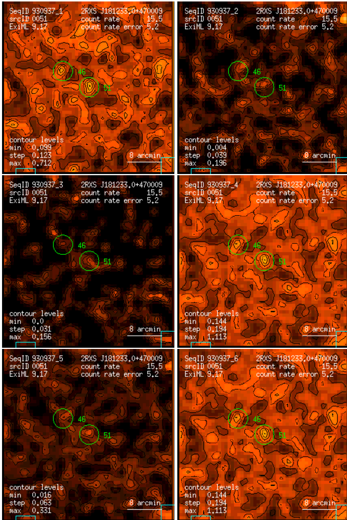
Figure 51: RASS 930937: detection 0051: band rate images, Gaussian filter: (1) PSPC channels 11 – 41, (2) 52 – 90, (3) 91 – 201, (4) 11 – 235, (5) 52 – 201, (6) 11 – 201. Broad band rates in counts/ks. Band rate contour levels in counts/ks/arcmin 2 .
