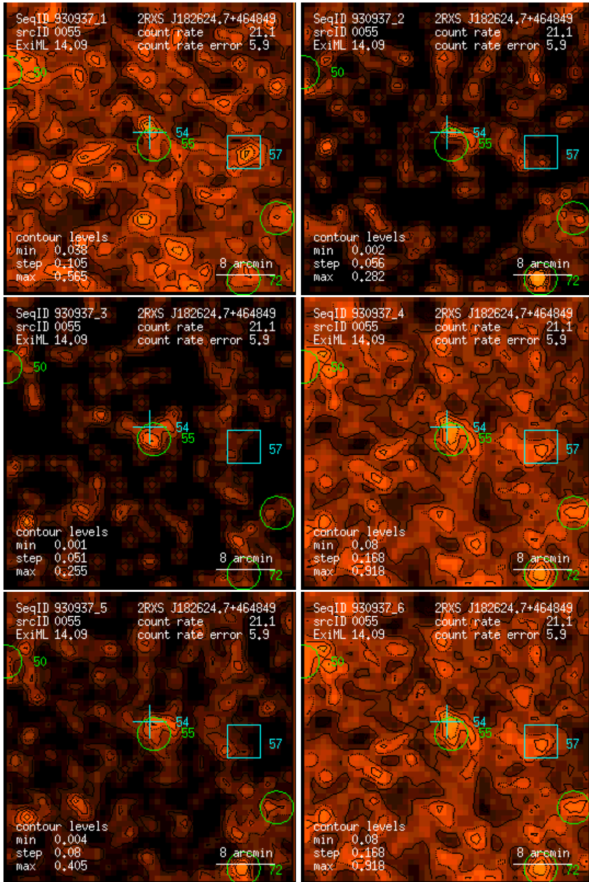
Figure 55: RASS 930937: detection 0055: band rate images, Gaussian filter: (1) PSPC channels 11 – 41, (2) 52 – 90, (3) 91 – 201, (4) 11 – 235, (5) 52 – 201, (6) 11 – 201. Broad band rates in counts/ks. Band rate contour levels in counts/ks/arcmin 2 .
