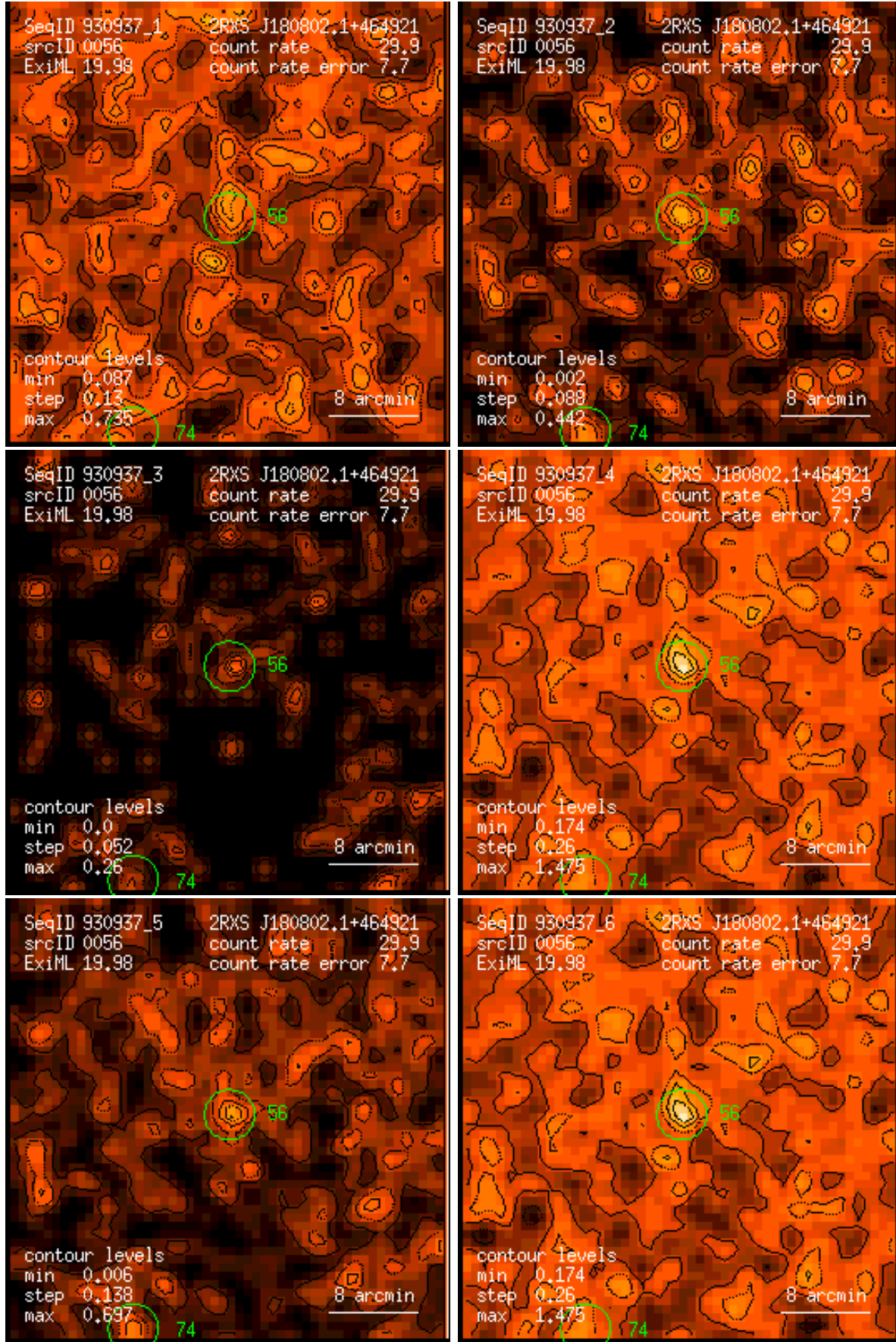
Figure 56: RASS 930937: detection 0056: band rate images, Gaussian filter: (1) PSPC channels 11 – 41, (2) 52 – 90, (3) 91 – 201, (4) 11 – 235, (5) 52 – 201, (6) 11 – 201. Broad band rates in counts/ks. Band rate contour levels in counts/ks/arcmin 2 .
