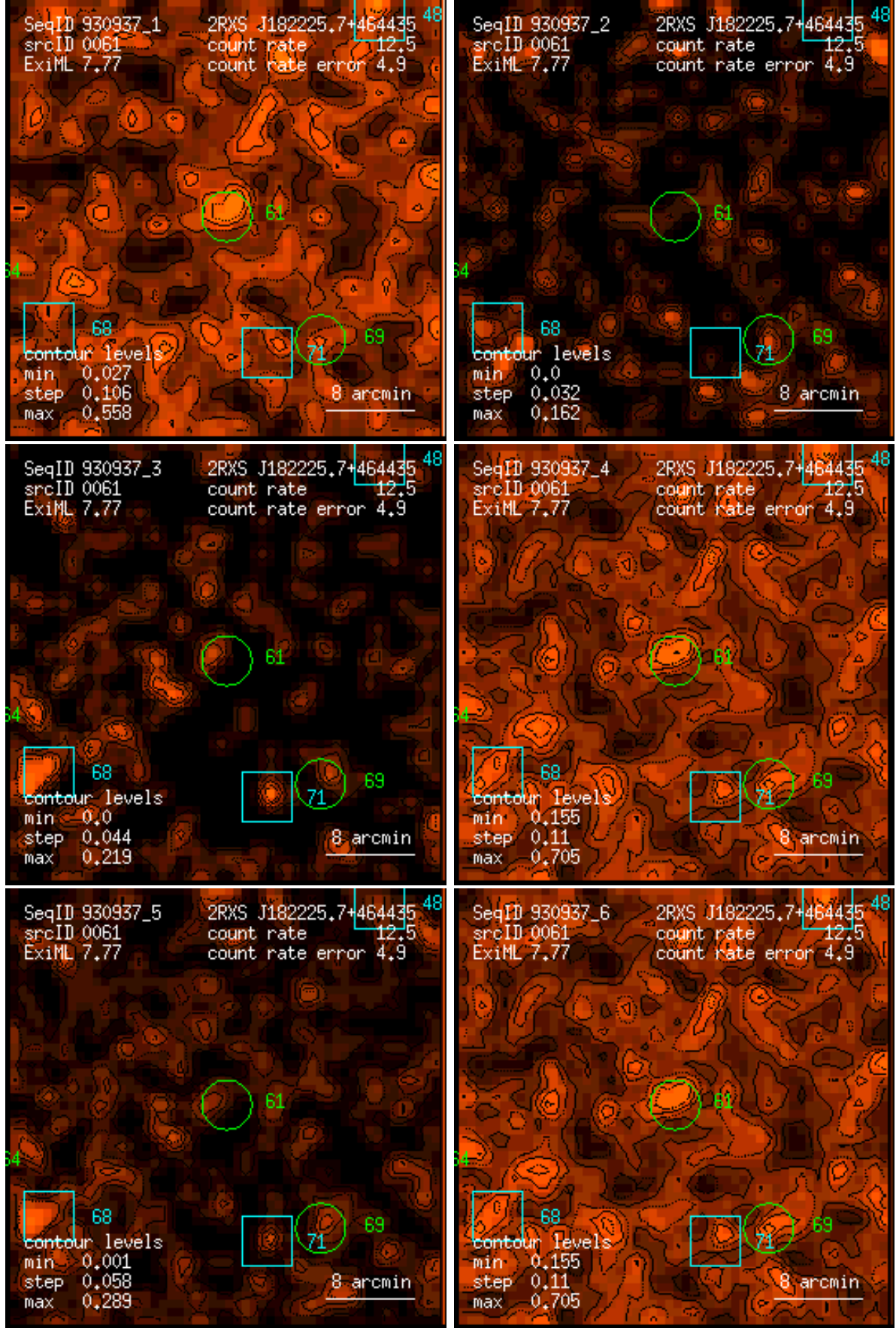
Figure 61: RASS 930937: detection 0061: band rate images, Gaussian filter: (1) PSPC channels 11 – 41, (2) 52 – 90, (3) 91 – 201, (4) 11 – 235, (5) 52 – 201, (6) 11 – 201. Broad band rates in counts/ks. Band rate contour levels in counts/ks/arcmin 2 .
