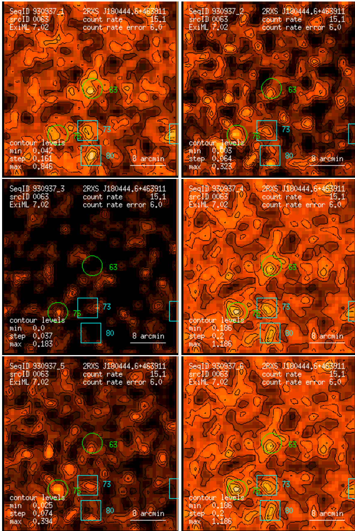
Figure 63: RASS 930937: detection 0063: band rate images, Gaussian filter: (1) PSPC channels 11 – 41, (2) 52 – 90, (3) 91 – 201, (4) 11 – 235, (5) 52 – 201, (6) 11 – 201. Broad band rates in counts/ks. Band rate contour levels in counts/ks/arcmin 2 .
