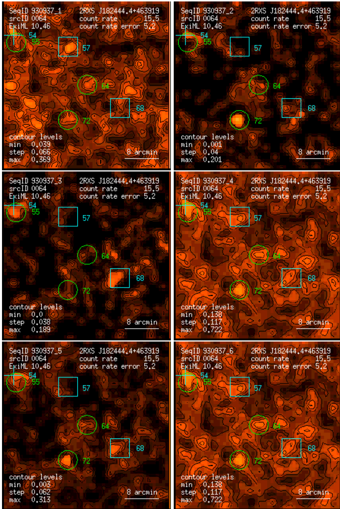
Figure 64: RASS 930937: detection 0064: band rate images, Gaussian filter: (1) PSPC channels 11 – 41, (2) 52 – 90, (3) 91 – 201, (4) 11 – 235, (5) 52 – 201, (6) 11 – 201. Broad band rates in counts/ks. Band rate contour levels in counts/ks/arcmin 2 .
