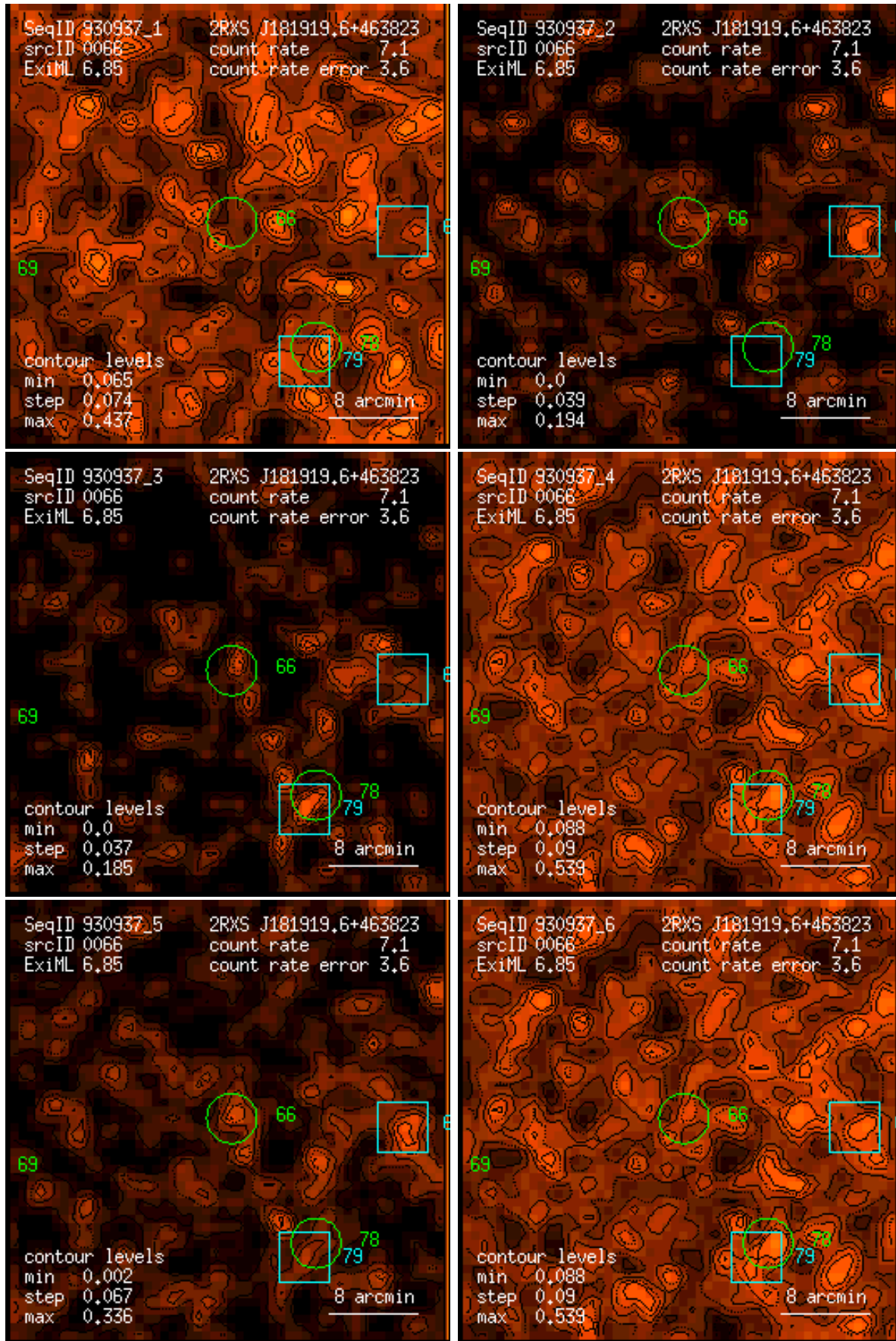
Figure 66: RASS 930937: detection 0066: band rate images, Gaussian filter: (1) PSPC channels 11 – 41, (2) 52 – 90, (3) 91 – 201, (4) 11 – 235, (5) 52 – 201, (6) 11 – 201. Broad band rates in counts/ks. Band rate contour levels in counts/ks/arcmin 2 .
