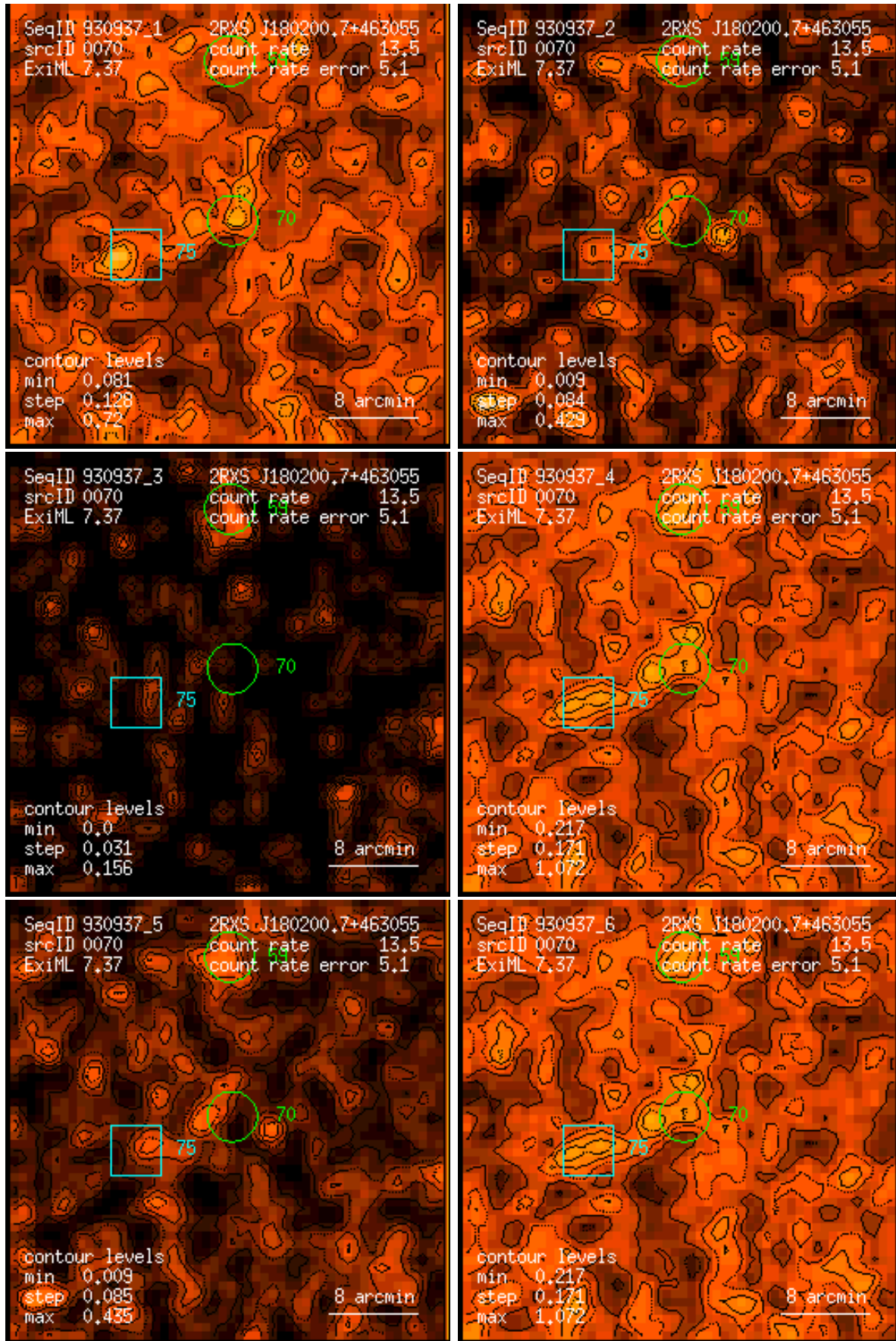
Figure 70: RASS 930937: detection 0070: band rate images, Gaussian filter: (1) PSPC channels 11 – 41, (2) 52 – 90, (3) 91 – 201, (4) 11 – 235, (5) 52 – 201, (6) 11 – 201. Broad band rates in counts/ks. Band rate contour levels in counts/ks/arcmin 2 .
