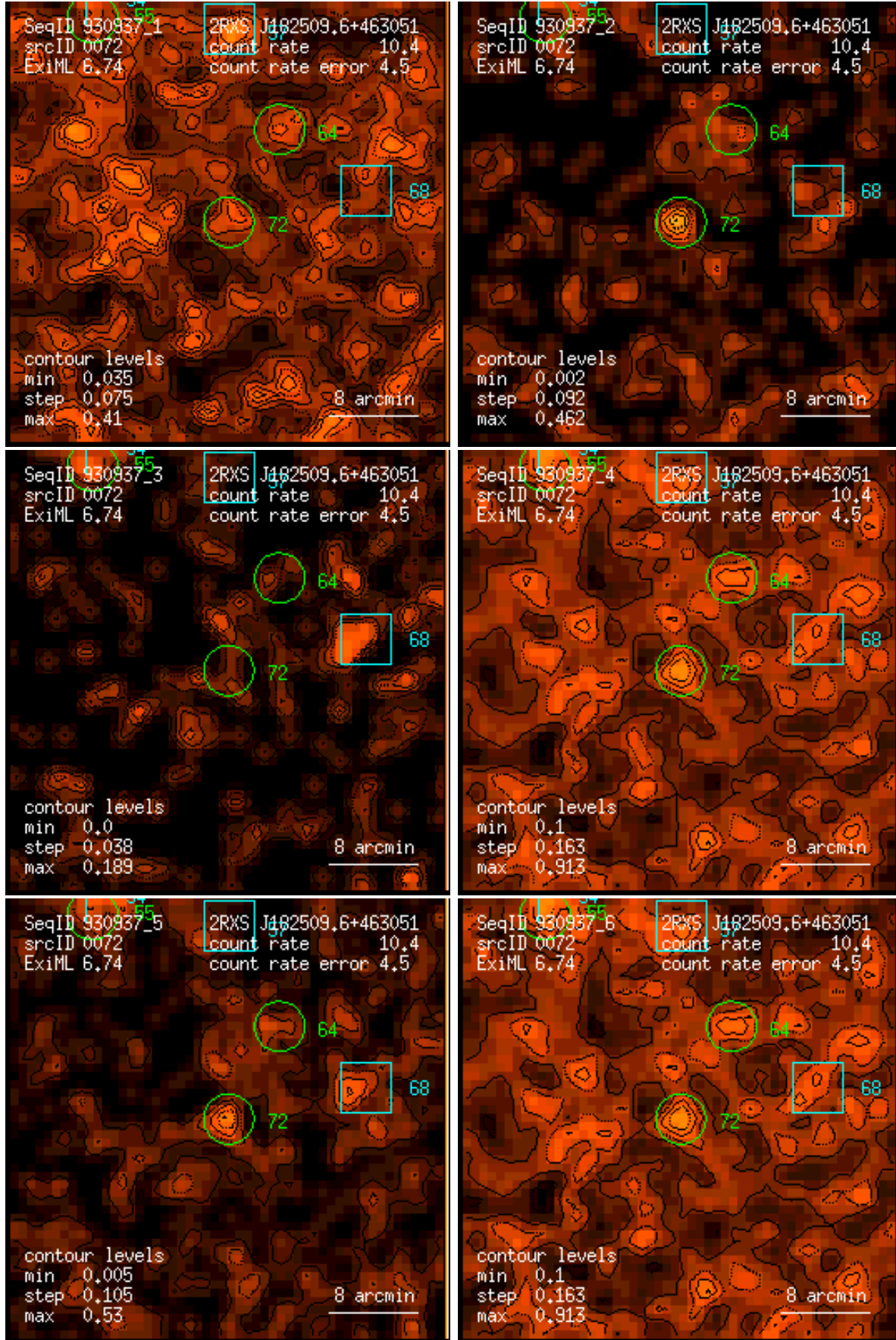
Figure 72: RASS 930937: detection 0072: band rate images, Gaussian filter: (1) PSPC channels 11 – 41, (2) 52 – 90, (3) 91 – 201, (4) 11 – 235, (5) 52 – 201, (6) 11 – 201. Broad band rates in counts/ks. Band rate contour levels in counts/ks/arcmin 2 .
