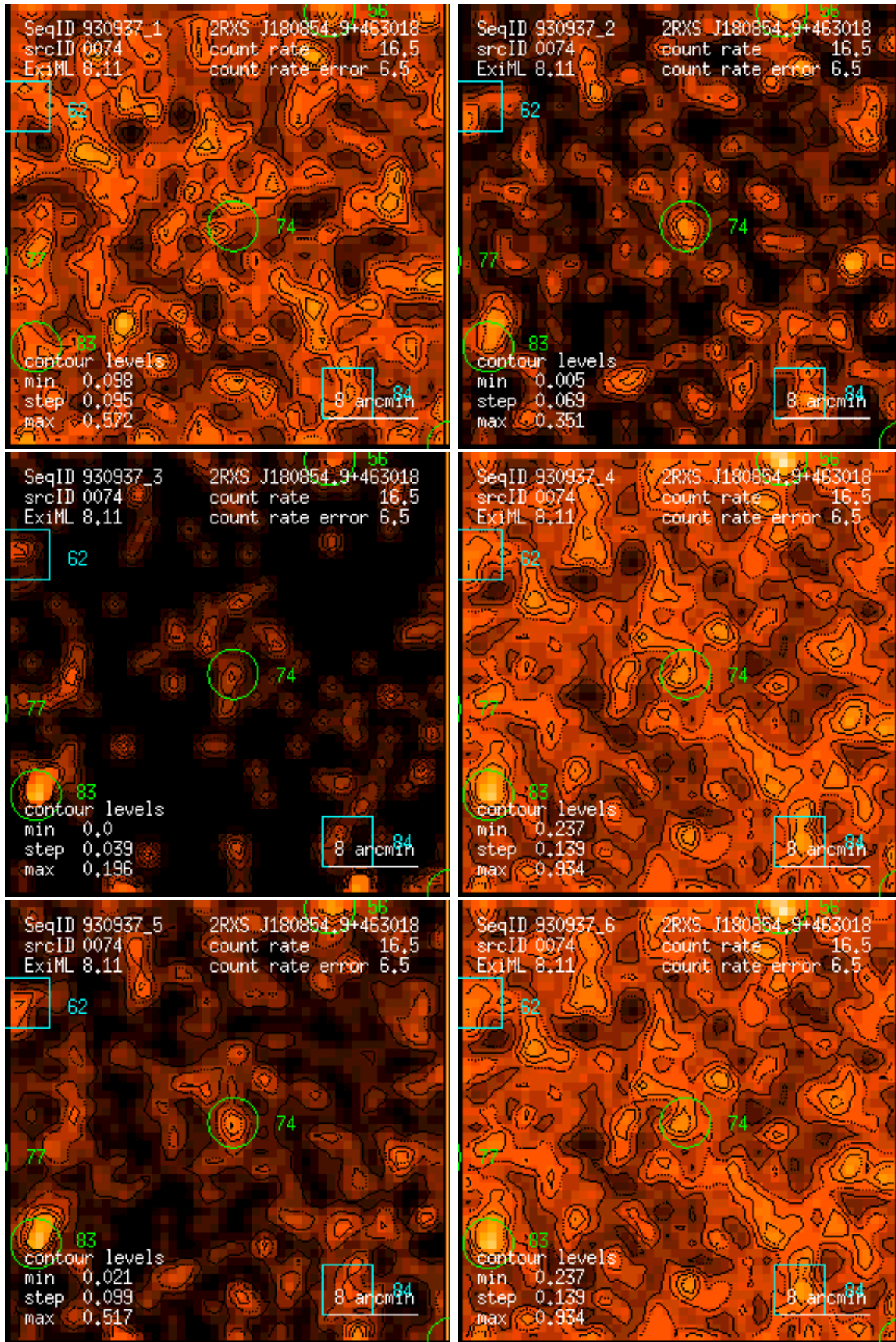
Figure 74: RASS 930937: detection 0074: band rate images, Gaussian filter: (1) PSPC channels 11 – 41, (2) 52 – 90, (3) 91 – 201, (4) 11 – 235, (5) 52 – 201, (6) 11 – 201. Broad band rates in counts/ks. Band rate contour levels in counts/ks/arcmin 2 .
