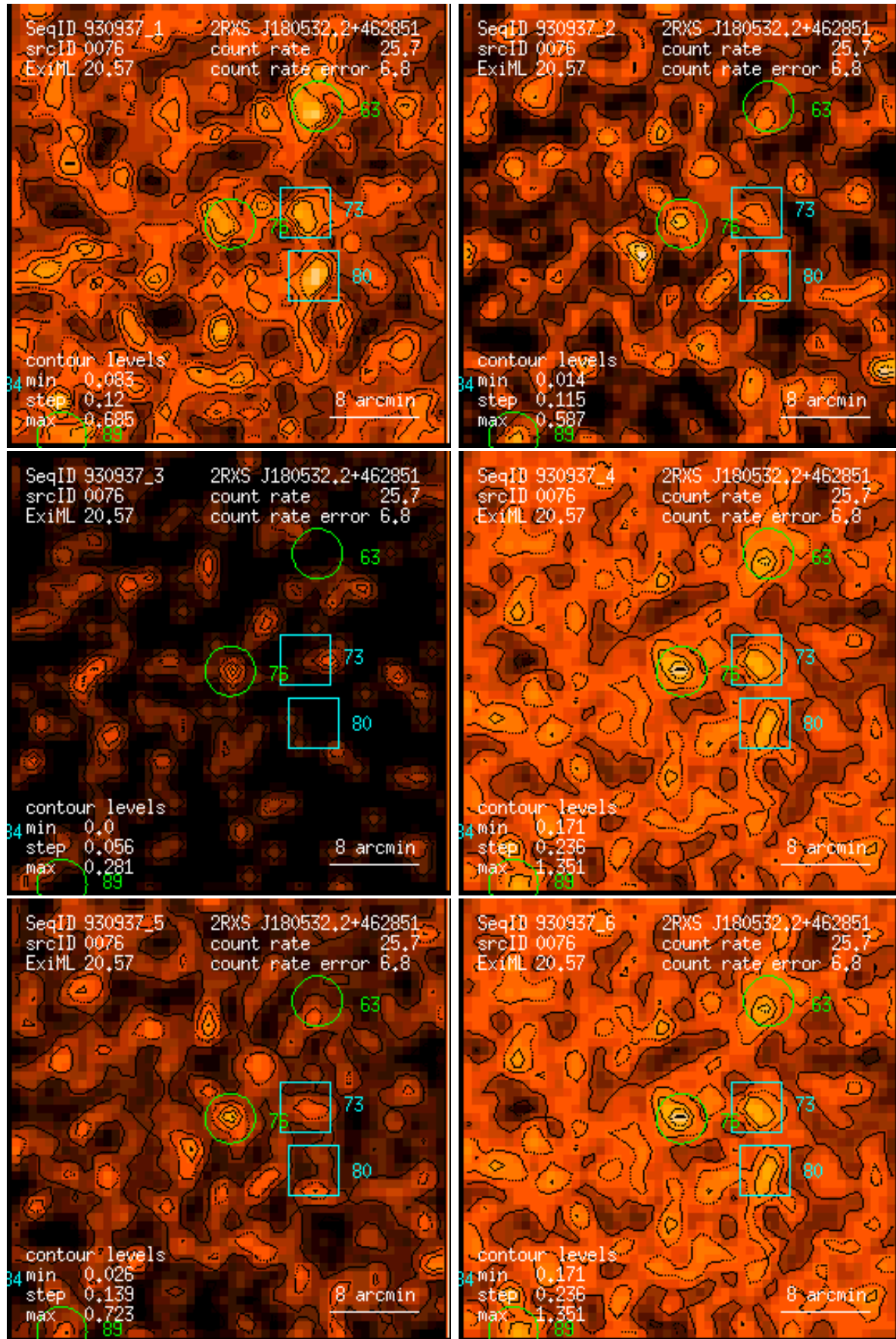
Figure 76: RASS 930937: detection 0076: band rate images, Gaussian filter: (1) PSPC channels 11 – 41, (2) 52 – 90, (3) 91 – 201, (4) 11 – 235, (5) 52 – 201, (6) 11 – 201. Broad band rates in counts/ks. Band rate contour levels in counts/ks/arcmin 2 .
