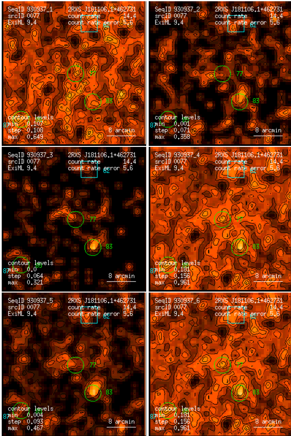
Figure 77: RASS 930937: detection 0077: band rate images, Gaussian filter: (1) PSPC channels 11 – 41, (2) 52 – 90, (3) 91 – 201, (4) 11 – 235, (5) 52 – 201, (6) 11 – 201. Broad band rates in counts/ks. Band rate contour levels in counts/ks/arcmin 2 .
