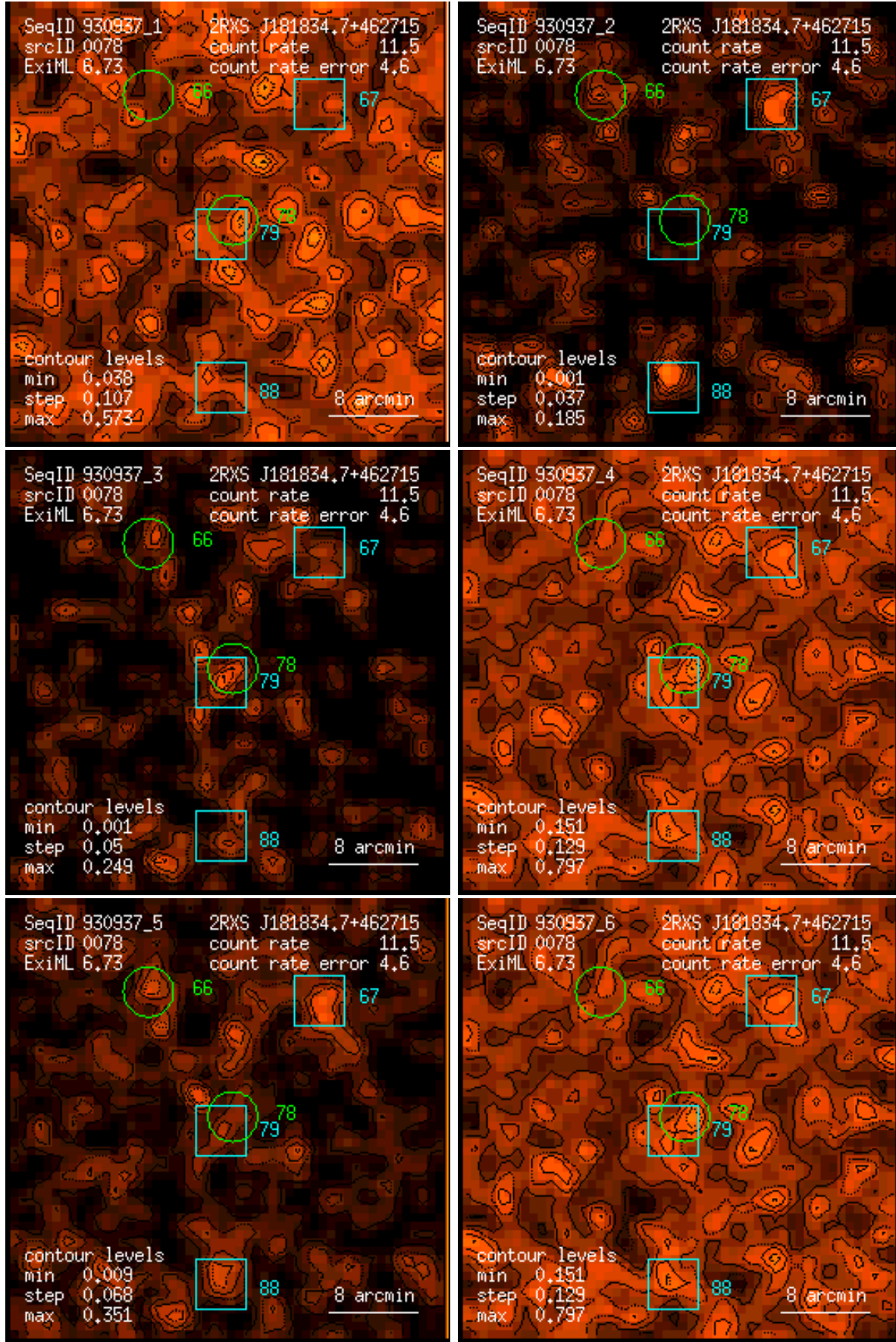
Figure 78: RASS 930937: detection 0078: band rate images, Gaussian filter: (1) PSPC channels 11 – 41, (2) 52 – 90, (3) 91 – 201, (4) 11 – 235, (5) 52 – 201, (6) 11 – 201. Broad band rates in counts/ks. Band rate contour levels in counts/ks/arcmin 2 .
