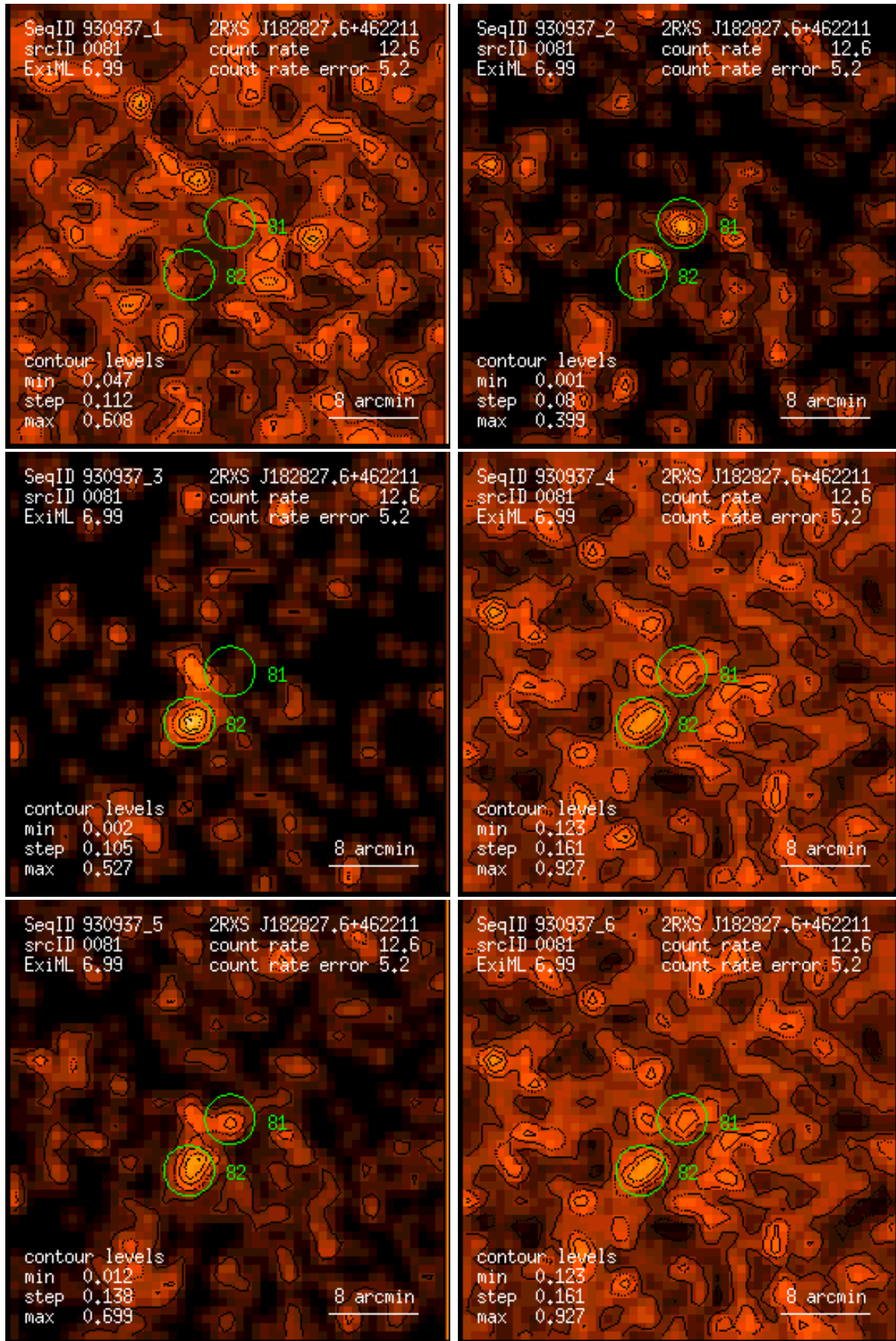
Figure 81: RASS 930937: detection 0081: band rate images, Gaussian filter: (1) PSPC channels 11 – 41, (2) 52 – 90, (3) 91 – 201, (4) 11 – 235, (5) 52 – 201, (6) 11 – 201. Broad band rates in counts/ks. Band rate contour levels in counts/ks/arcmin 2 .
