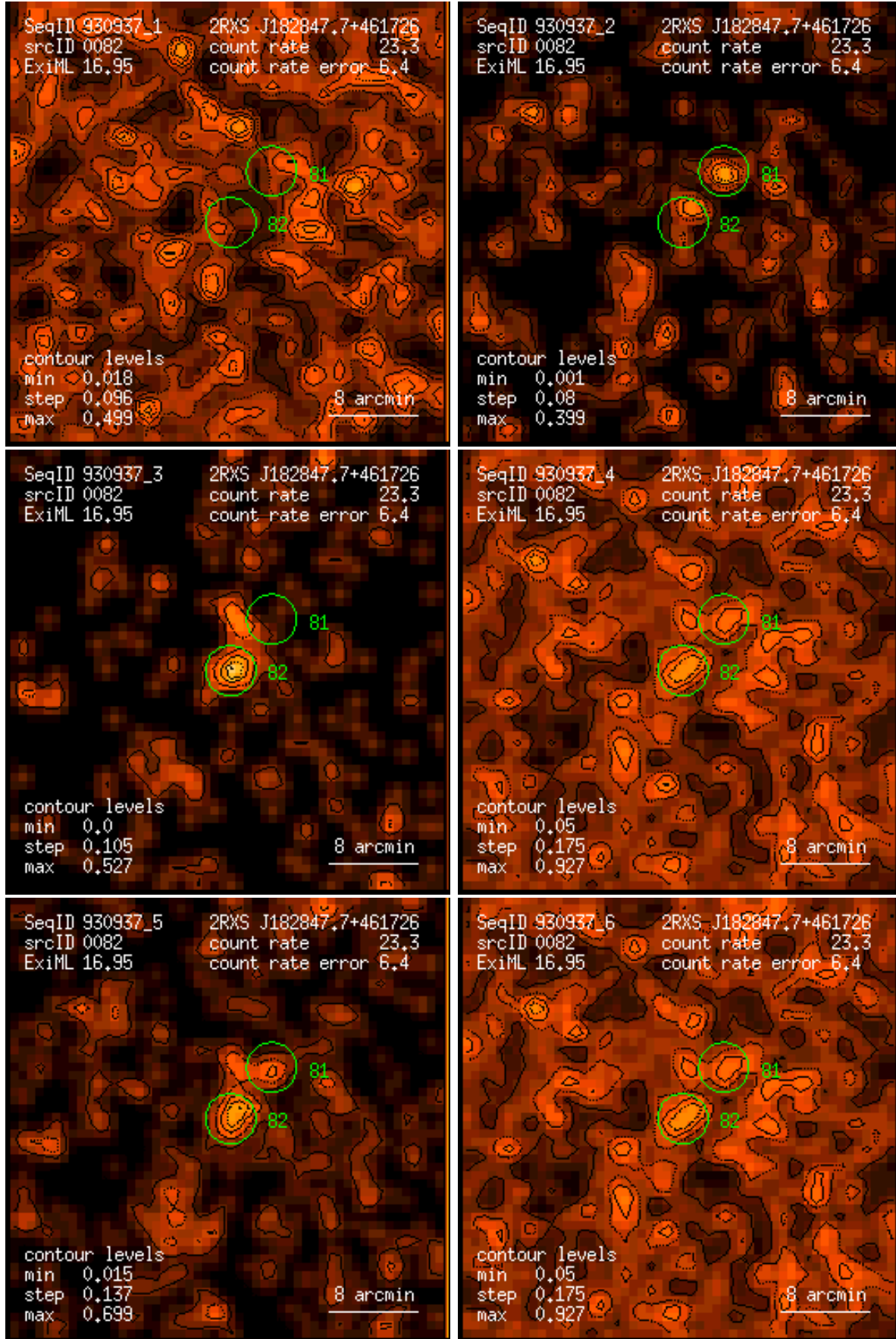
Figure 82: RASS 930937: detection 0082: band rate images, Gaussian filter: (1) PSPC channels 11 – 41, (2) 52 – 90, (3) 91 – 201, (4) 11 – 235, (5) 52 – 201, (6) 11 – 201. Broad band rates in counts/ks. Band rate contour levels in counts/ks/arcmin 2 .
