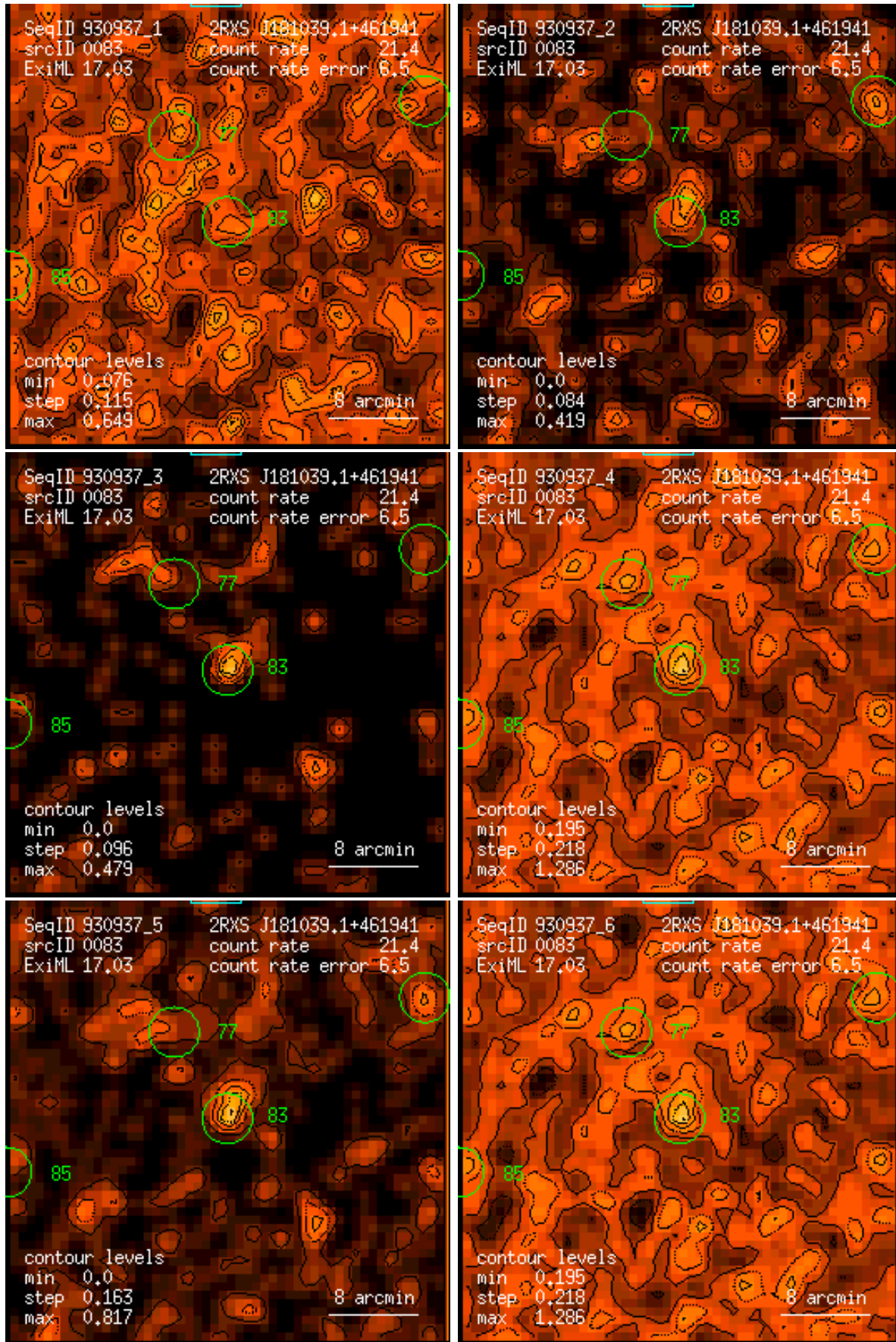
Figure 83: RASS 930937: detection 0083: band rate images, Gaussian filter: (1) PSPC channels 11 – 41, (2) 52 – 90, (3) 91 – 201, (4) 11 – 235, (5) 52 – 201, (6) 11 – 201. Broad band rates in counts/ks. Band rate contour levels in counts/ks/arcmin 2 .
