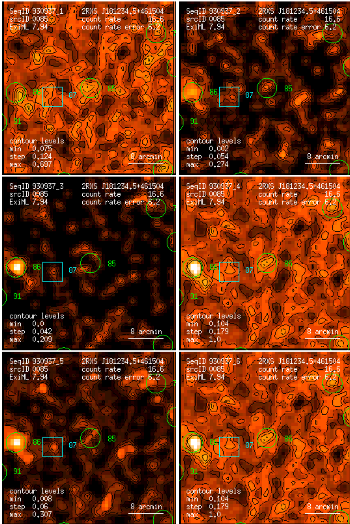
Figure 85: RASS 930937: detection 0085: band rate images, Gaussian filter: (1) PSPC channels 11 – 41, (2) 52 – 90, (3) 91 – 201, (4) 11 – 235, (5) 52 – 201, (6) 11 – 201. Broad band rates in counts/ks. Band rate contour levels in counts/ks/arcmin 2 .
