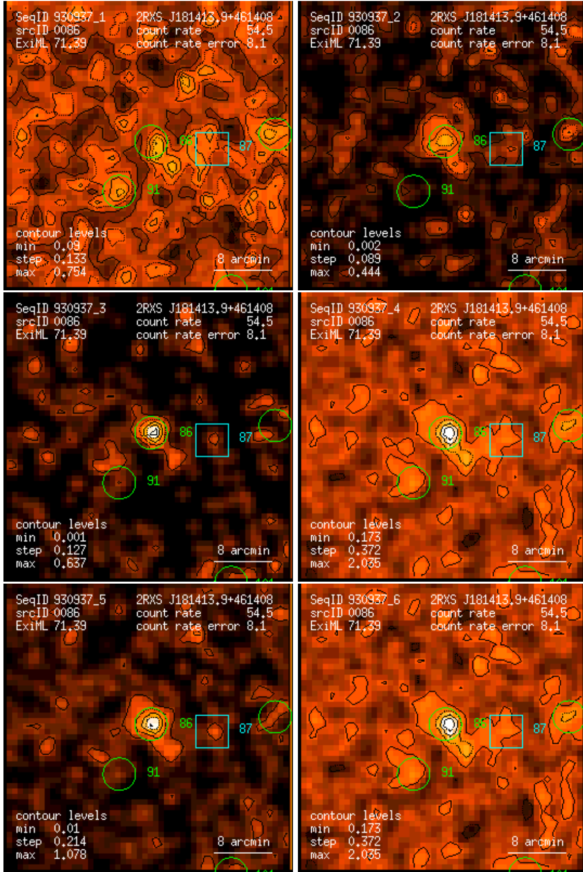
Figure 86: RASS 930937: detection 0086: band rate images, Gaussian filter: (1) PSPC channels 11 – 41, (2) 52 – 90, (3) 91 – 201, (4) 11 – 235, (5) 52 – 201, (6) 11 – 201. Broad band rates in counts/ks. Band rate contour levels in counts/ks/arcmin 2 .
