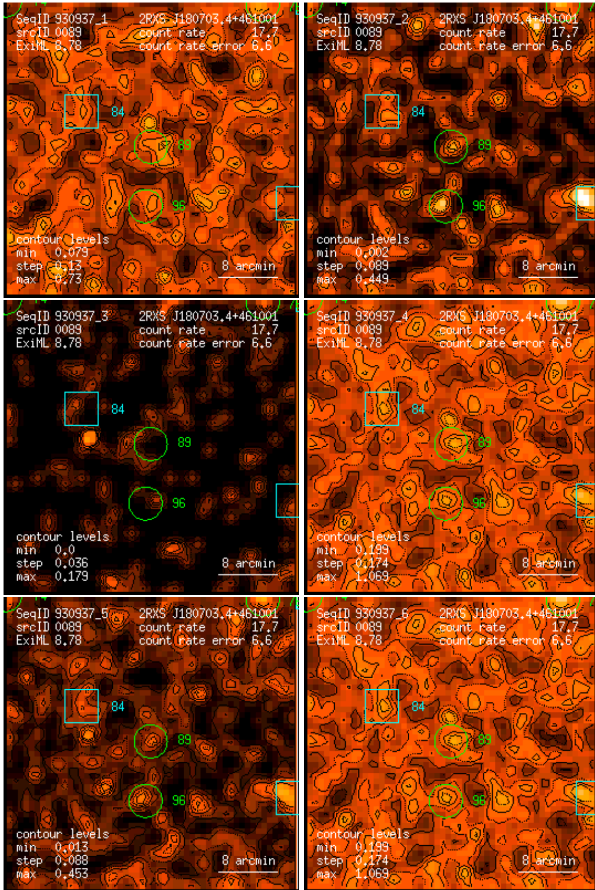
Figure 89: RASS 930937: detection 0089: band rate images, Gaussian filter: (1) PSPC channels 11 – 41, (2) 52 – 90, (3) 91 – 201, (4) 11 – 235, (5) 52 – 201, (6) 11 – 201. Broad band rates in counts/ks. Band rate contour levels in counts/ks/arcmin 2 .
