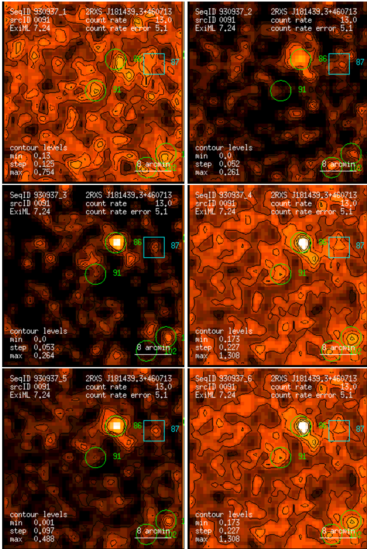
Figure 91: RASS 930937: detection 0091: band rate images, Gaussian filter: (1) PSPC channels 11 – 41, (2) 52 – 90, (3) 91 – 201, (4) 11 – 235, (5) 52 – 201, (6) 11 – 201. Broad band rates in counts/ks. Band rate contour levels in counts/ks/arcmin 2 .
