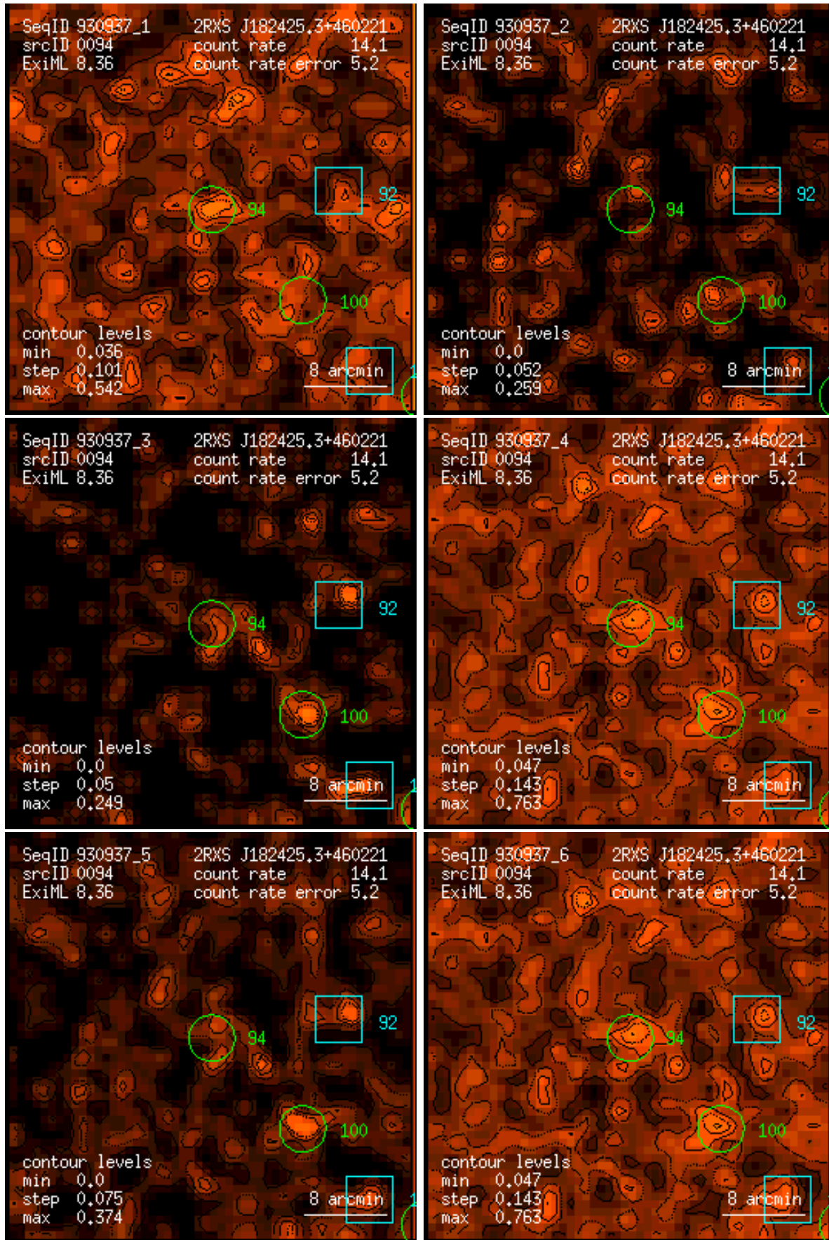
Figure 94: RASS 930937: detection 0094: band rate images, Gaussian filter: (1) PSPC channels 11 – 41, (2) 52 – 90, (3) 91 – 201, (4) 11 – 235, (5) 52 – 201, (6) 11 – 201. Broad band rates in counts/ks. Band rate contour levels in counts/ks/arcmin 2 .
