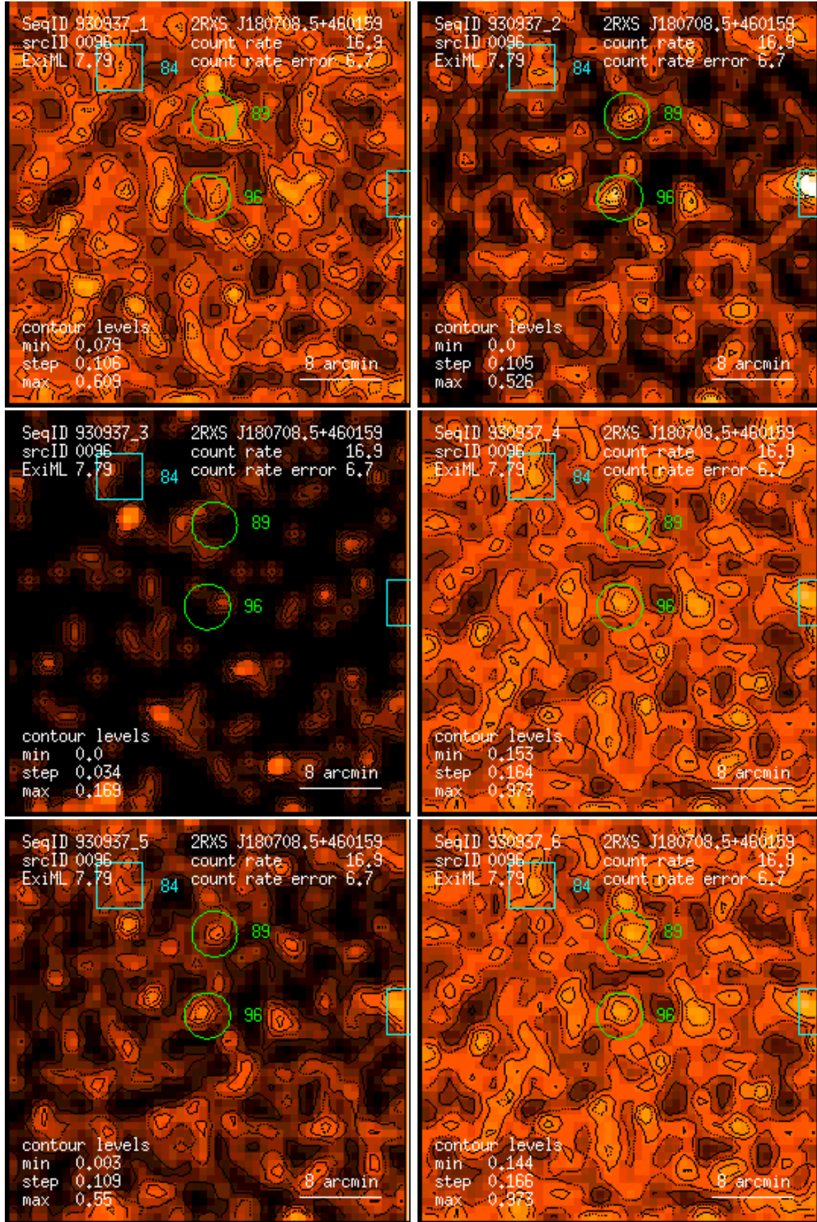
Figure 96: RASS 930937: detection 0096: band rate images, Gaussian filter: (1) PSPC channels 11 – 41, (2) 52 – 90, (3) 91 – 201, (4) 11 – 235, (5) 52 – 201, (6) 11 – 201. Broad band rates in counts/ks. Band rate contour levels in counts/ks/arcmin 2 .
