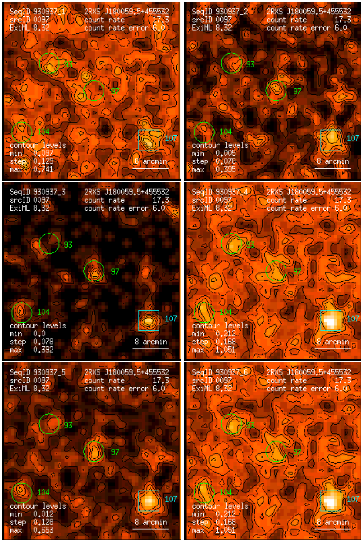
Figure 97: RASS 930937: detection 0097: band rate images, Gaussian filter: (1) PSPC channels 11 – 41, (2) 52 – 90, (3) 91 – 201, (4) 11 – 235, (5) 52 – 201, (6) 11 – 201. Broad band rates in counts/ks. Band rate contour levels in counts/ks/arcmin 2 .
