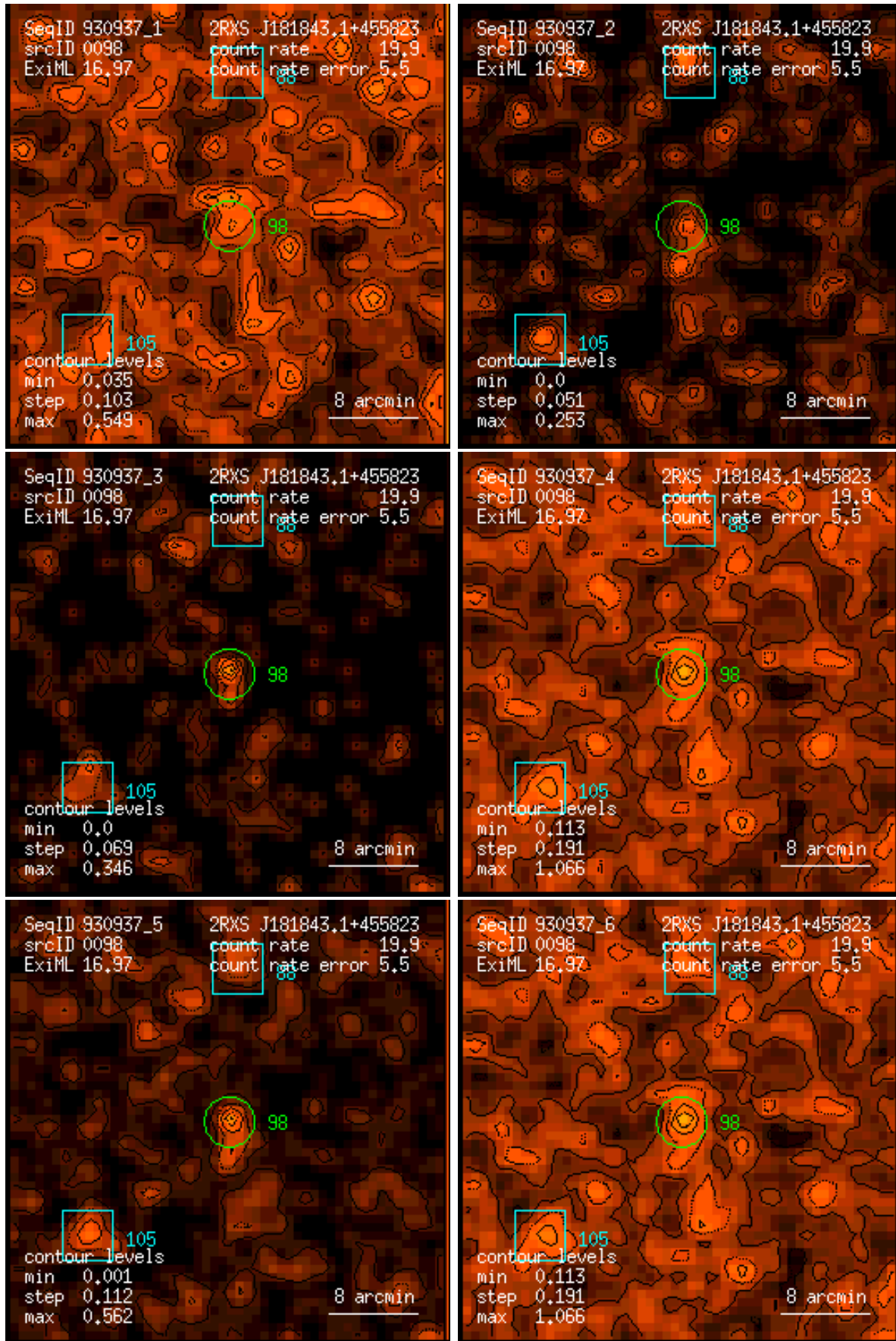
Figure 98: RASS 930937: detection 0098: band rate images, Gaussian filter: (1) PSPC channels 11 – 41, (2) 52 – 90, (3) 91 – 201, (4) 11 – 235, (5) 52 – 201, (6) 11 – 201. Broad band rates in counts/ks. Band rate contour levels in counts/ks/arcmin 2 .
