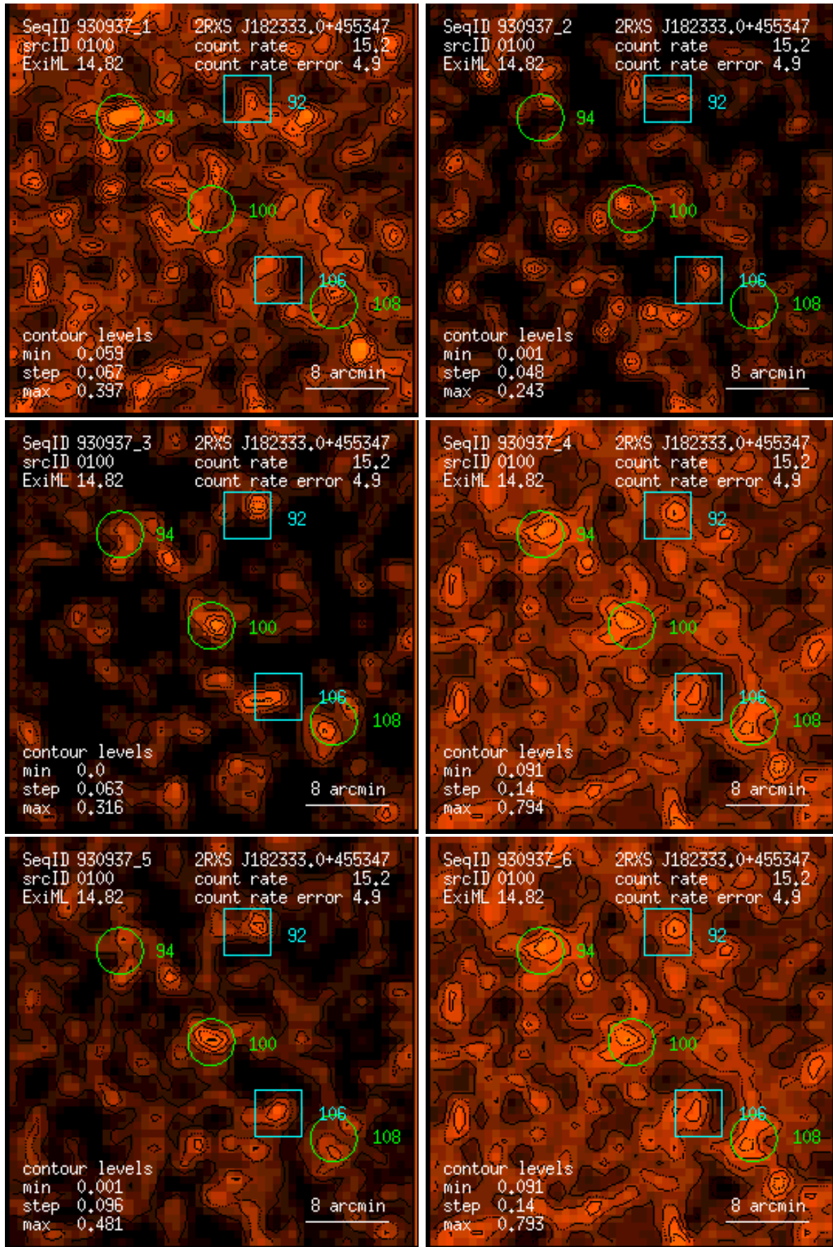
Figure 100: RASS 930937: detection 0100: band rate images, Gaussian filter: (1) PSPC channels 11 – 41, (2) 52 – 90, (3) 91 – 201, (4) 11 – 235, (5) 52 – 201, (6) 11 – 201. Broad band rates in counts/ks. Band rate contour levels in counts/ks/arcmin 2 .
