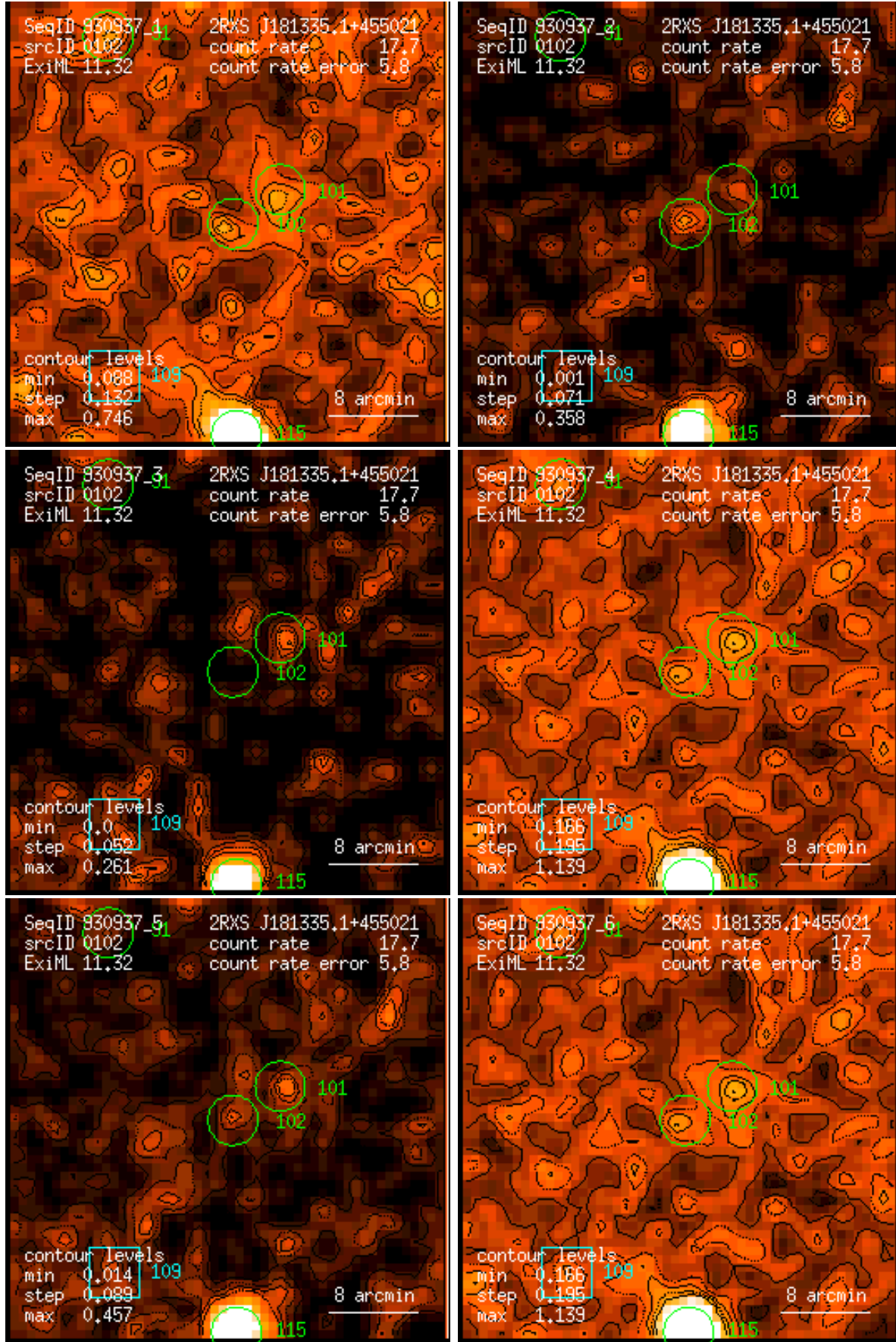
Figure 102: RASS 930937: detection 0102: band rate images, Gaussian filter: (1) PSPC channels 11 – 41, (2) 52 – 90, (3) 91 – 201, (4) 11 – 235, (5) 52 – 201, (6) 11 – 201. Broad band rates in counts/ks. Band rate contour levels in counts/ks/arcmin 2 .
