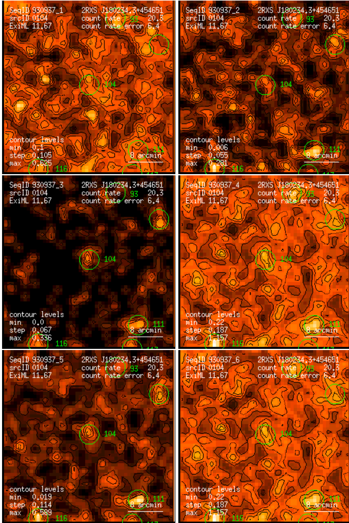
Figure 104: RASS 930937: detection 0104: band rate images, Gaussian filter: (1) PSPC channels 11 – 41, (2) 52 – 90, (3) 91 – 201, (4) 11 – 235, (5) 52 – 201, (6) 11 – 201. Broad band rates in counts/ks. Band rate contour levels in counts/ks/arcmin 2 .
