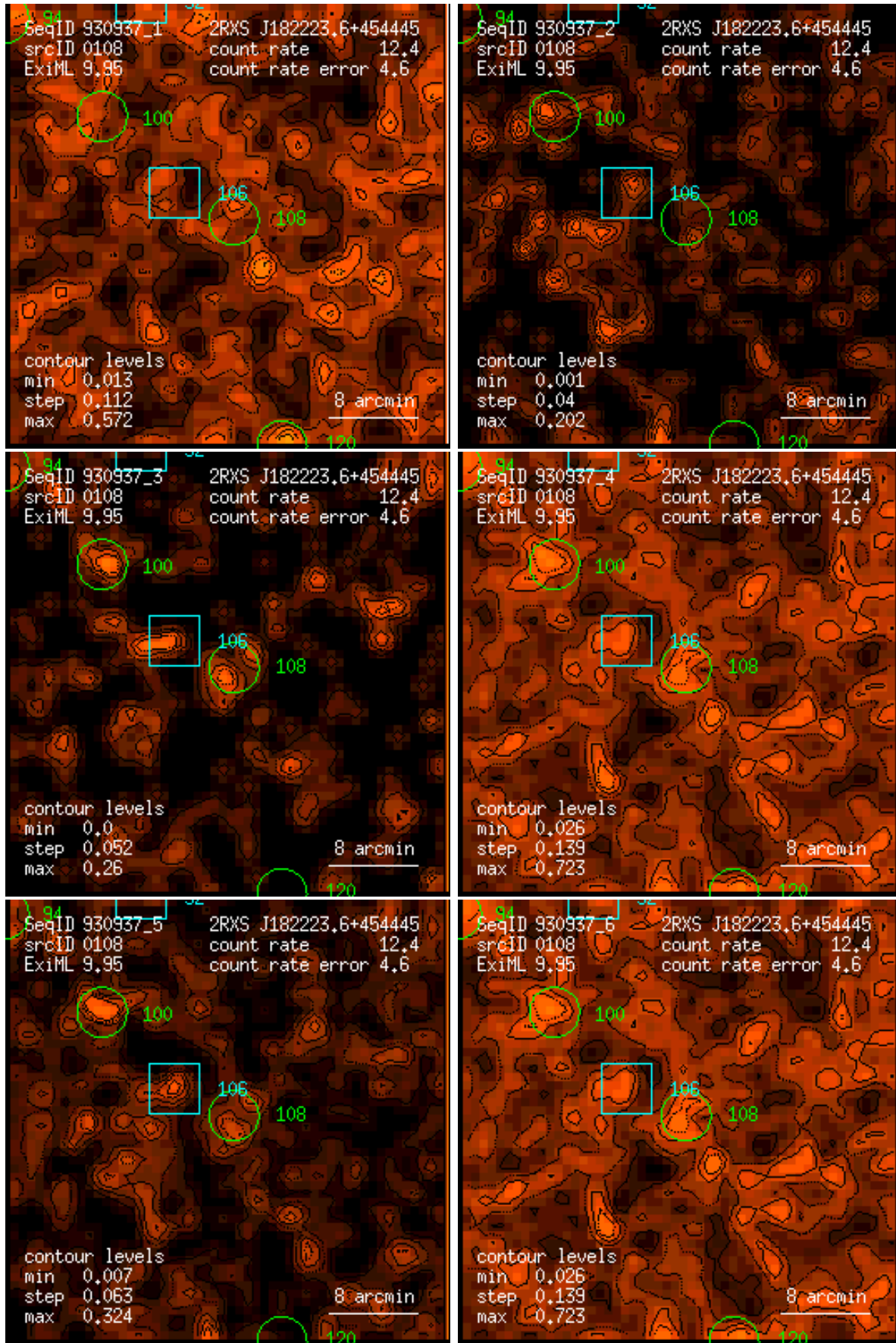
Figure 108: RASS 930937: detection 0108: band rate images, Gaussian filter: (1) PSPC channels 11 – 41, (2) 52 – 90, (3) 91 – 201, (4) 11 – 235, (5) 52 – 201, (6) 11 – 201. Broad band rates in counts/ks. Band rate contour levels in counts/ks/arcmin 2 .
