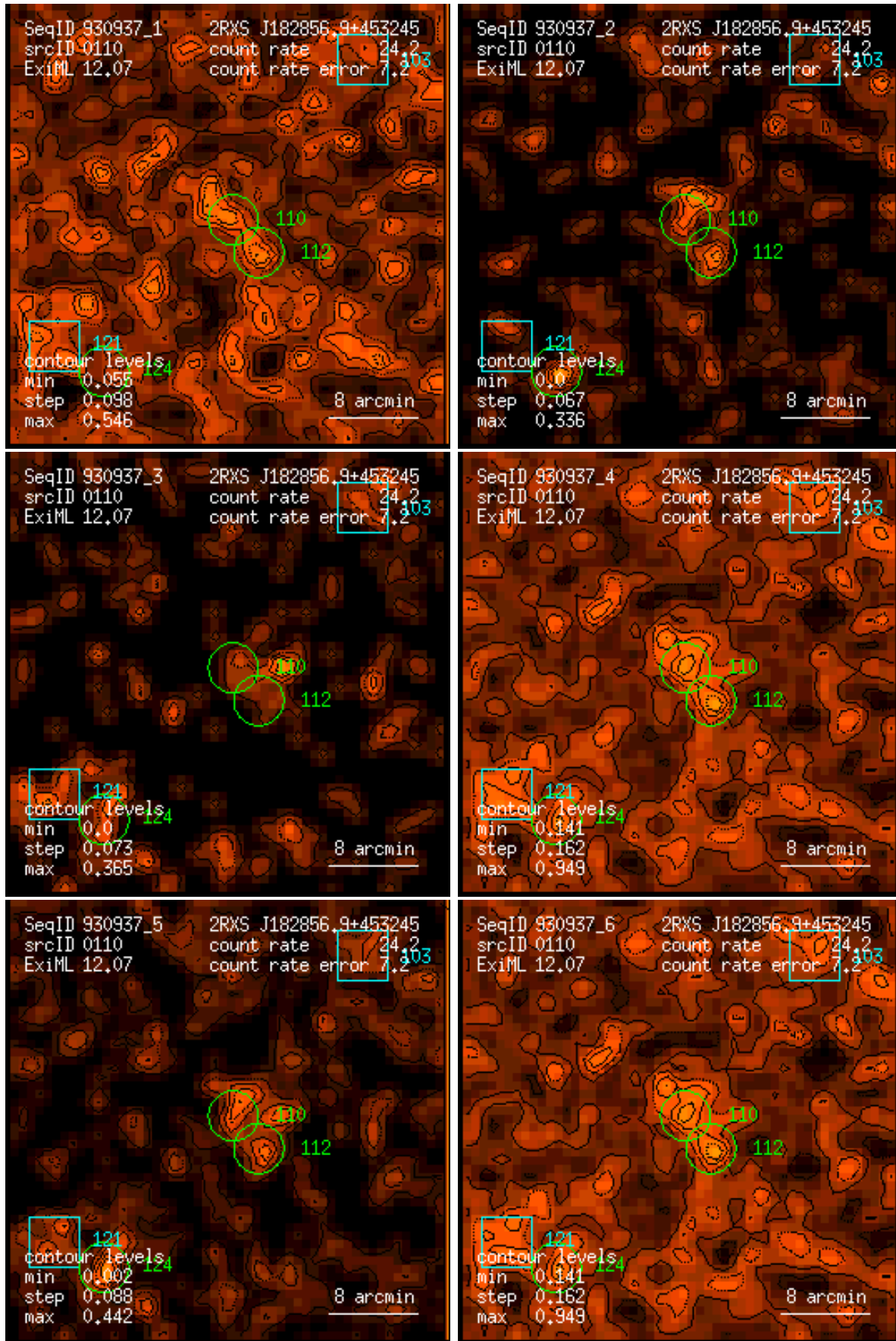
Figure 110: RASS 930937: detection 0110: band rate images, Gaussian filter: (1) PSPC channels 11 – 41, (2) 52 – 90, (3) 91 – 201, (4) 11 – 235, (5) 52 – 201, (6) 11 – 201. Broad band rates in counts/ks. Band rate contour levels in counts/ks/arcmin 2 .
